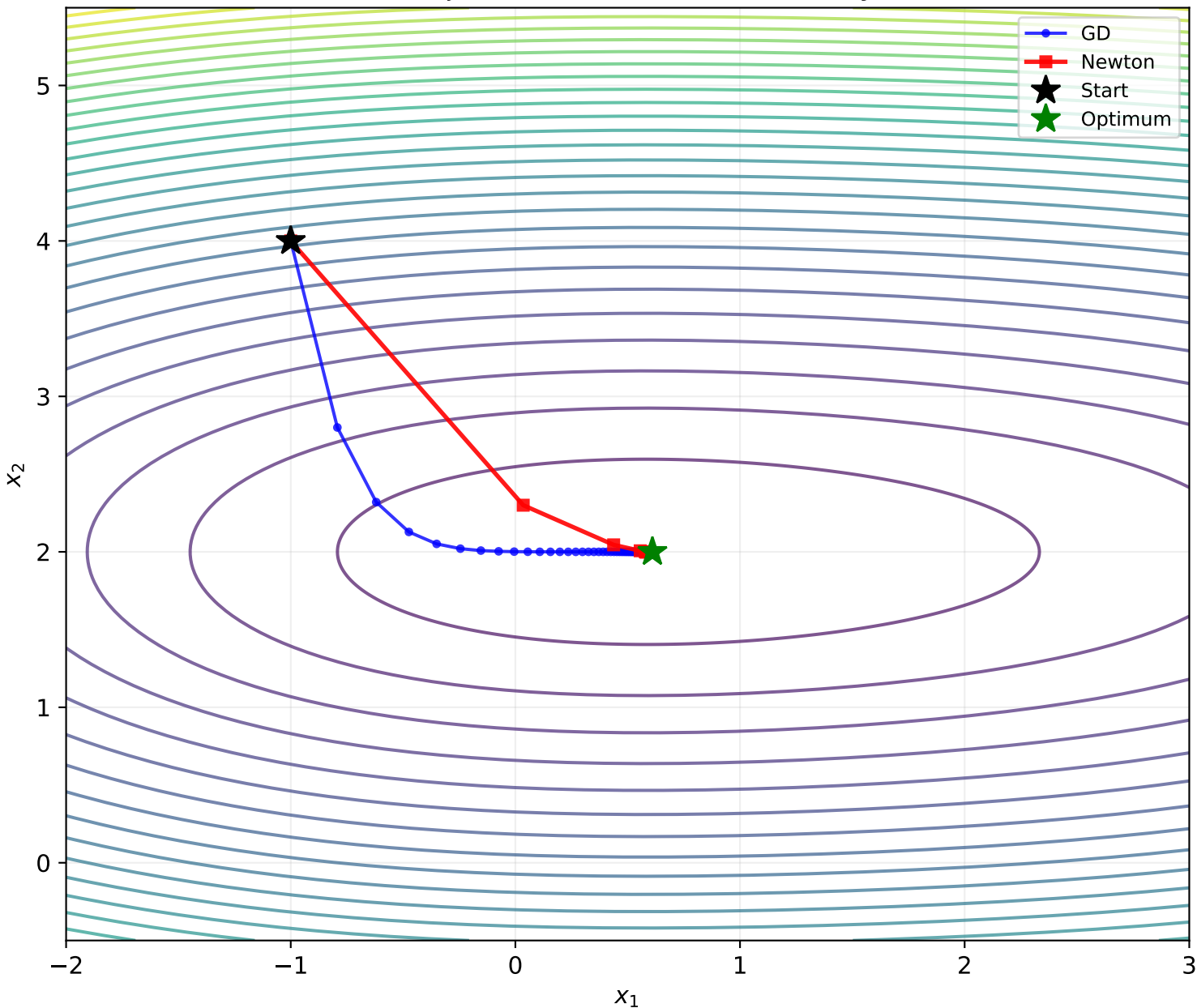
Q3: Newton vs GD Trajectories — Benchmark B (Toy Neural Network)
