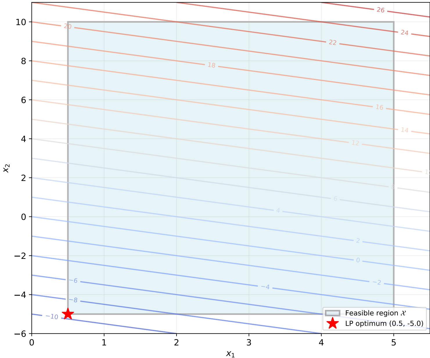
Q6-I: Linear Programme — f(x) = x_1 + 2x_2 , f^* = -9.5
