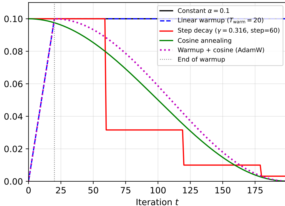
Learning Rate Schedules (linear scale)
