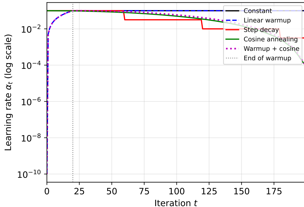
Learning Rate Schedules (log scale)
