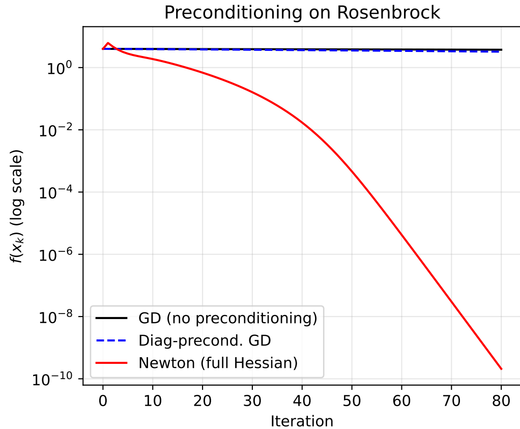
Effect of Preconditioning on Rosenbrock ( \kappa \approx 2504 )
