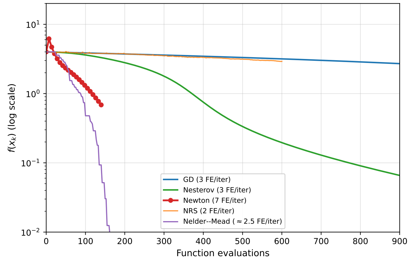
Oracle type comparison (cost-adjusted) vs function evaluations
