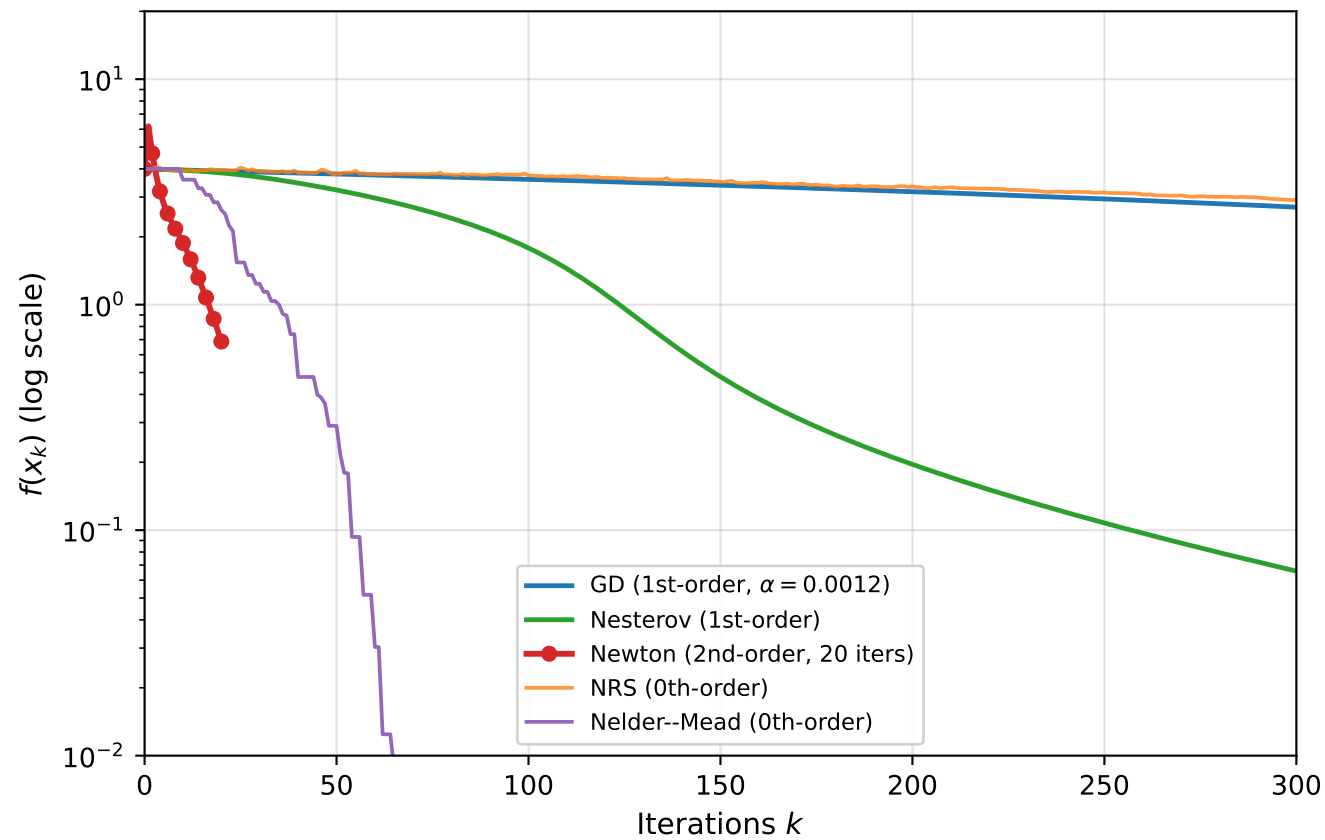
Oracle type comparison on Rosenbrock (Benchmark C, f^* = 0 )
