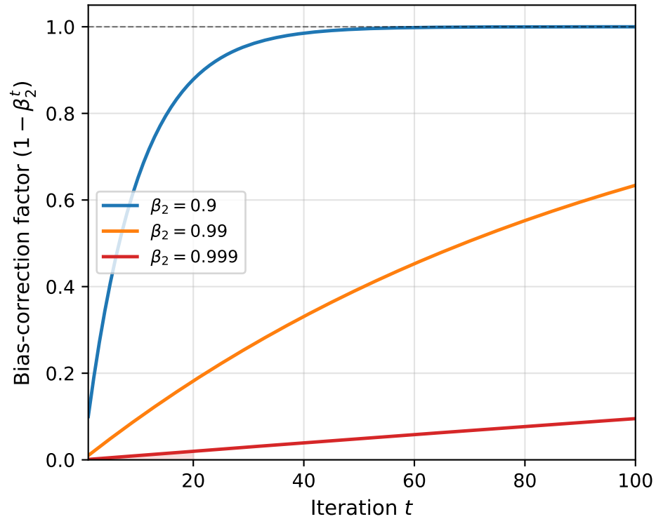
Bias correction warm-up speed for different \beta_2
