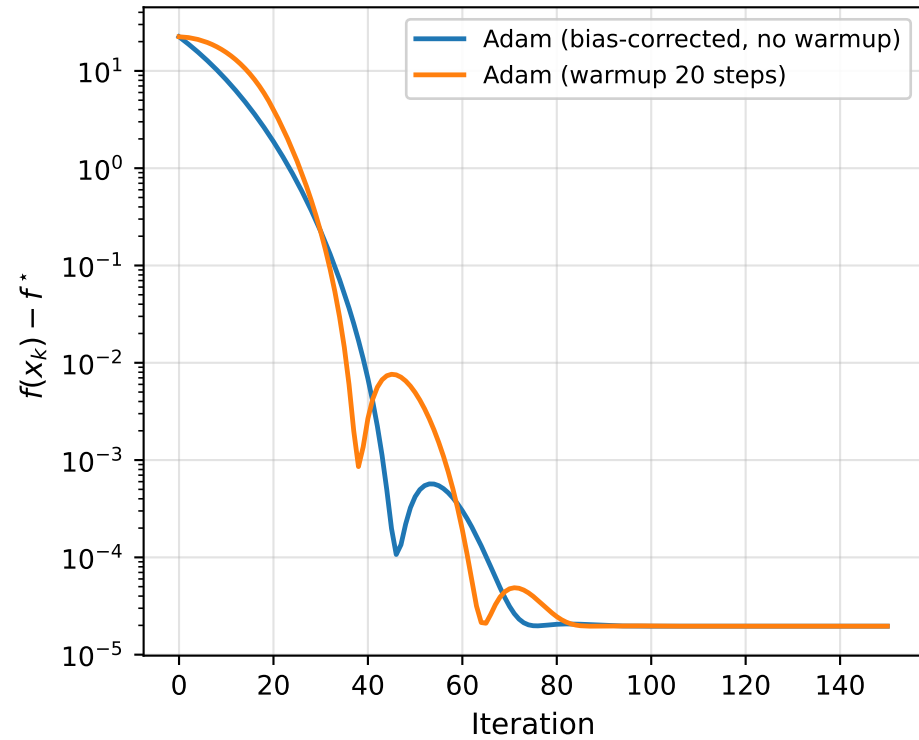
Adam variants on Benchmark B
