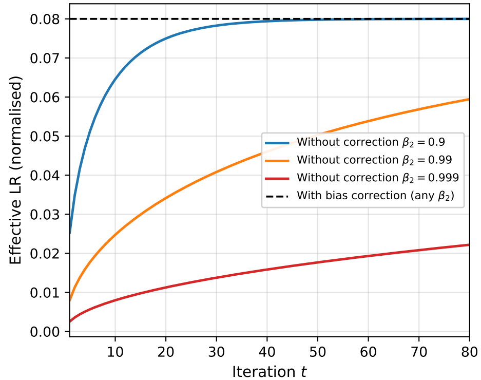
Bias correction effect on effective learning rate (early iterations)
