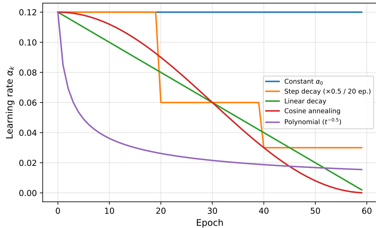
Learning-rate schedule comparison
