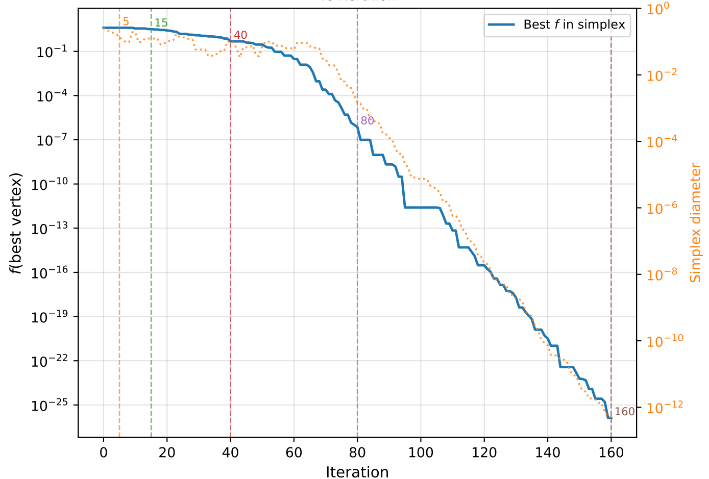
Convergence and simplex size vs iteration
