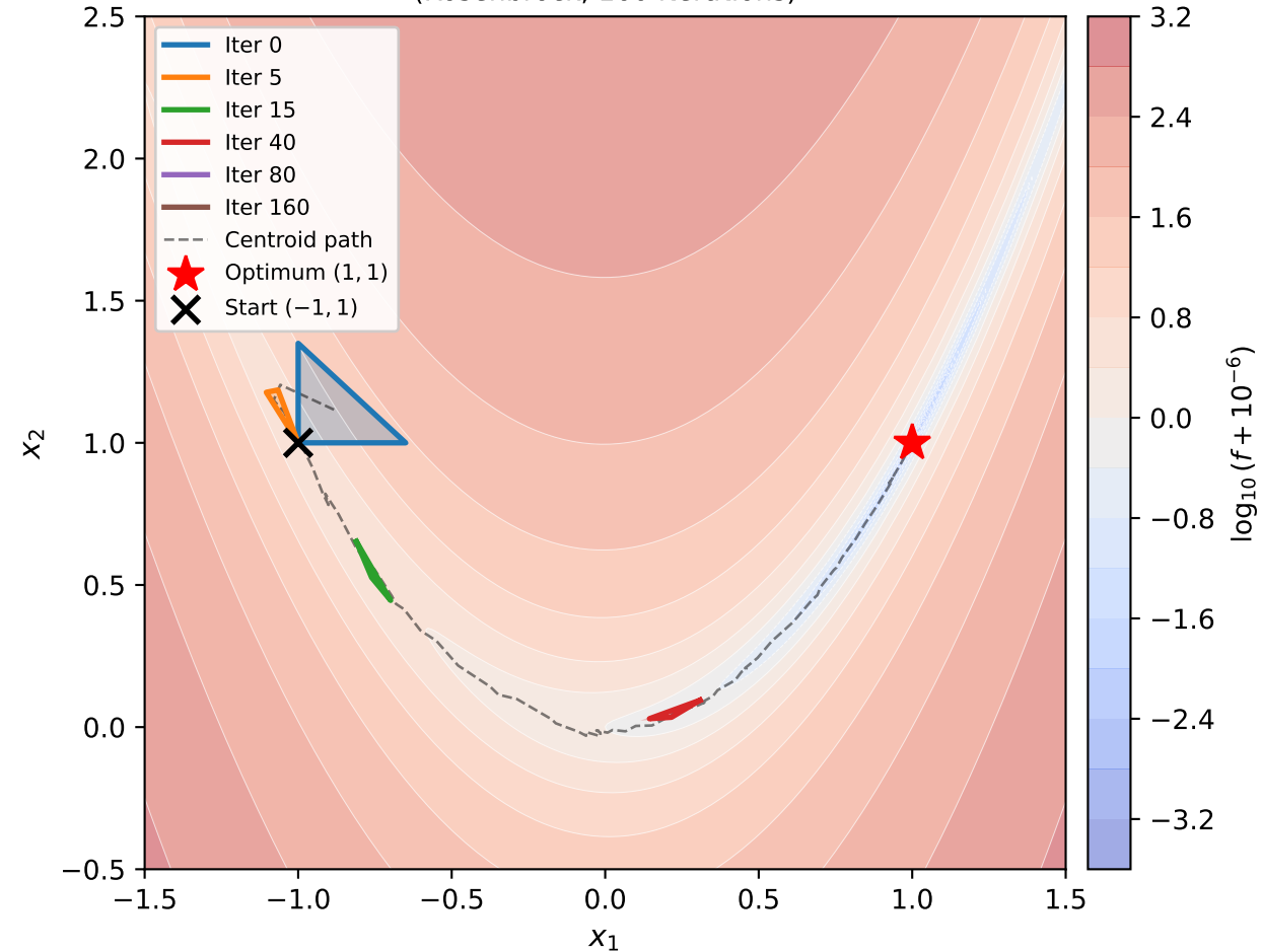
Nelder-Mead simplex evolution (Rosenbrock, 160 iterations)
