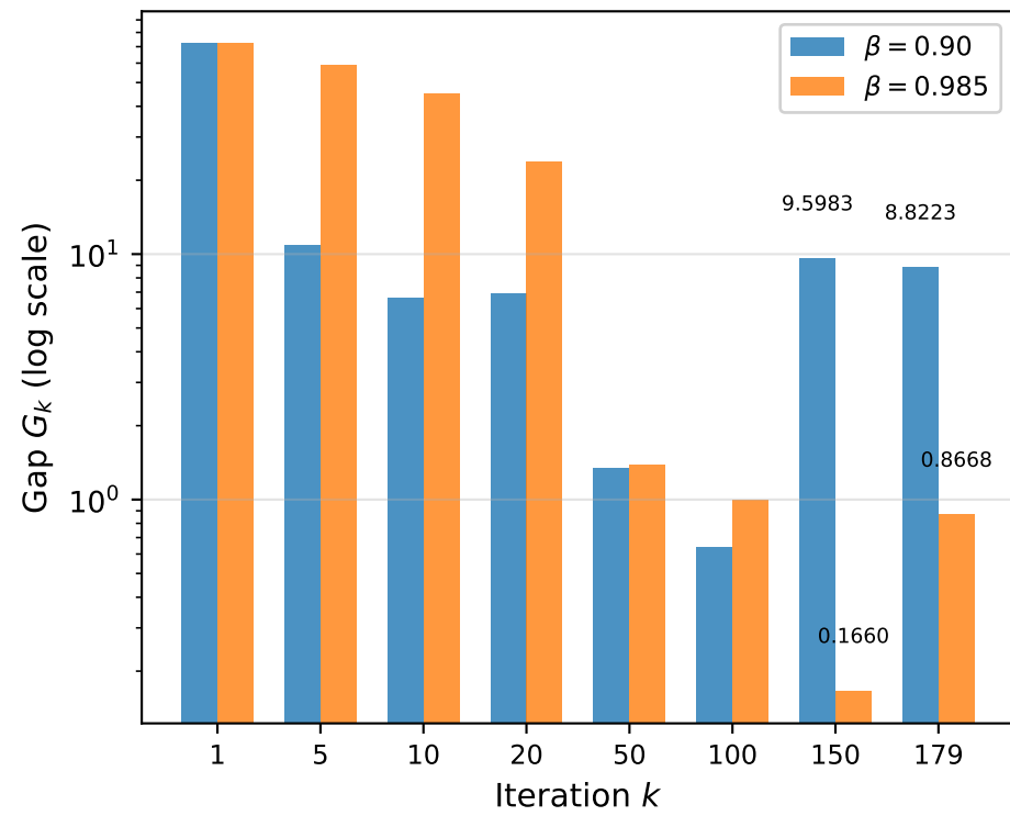
Gap values at selected iterations (Interior optimum, numerical)
