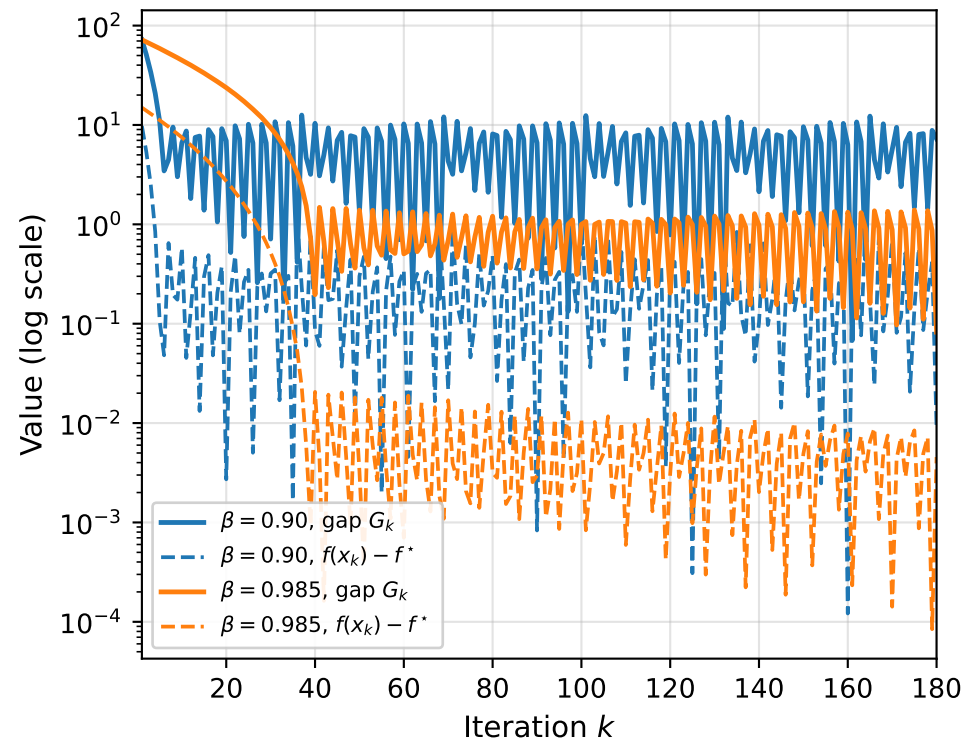
FW gap vs optimality gap (Interior optimum (1, 5))
