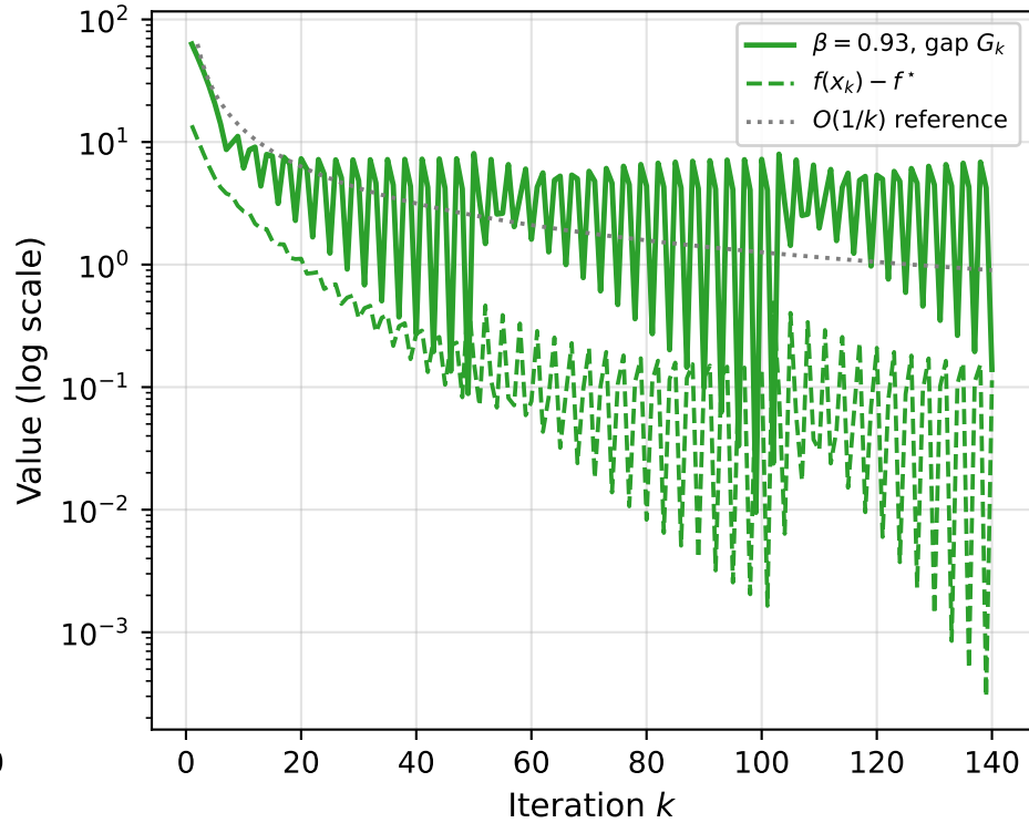
FW gap vs optimality gap (Boundary optimum (0.5, 0))
