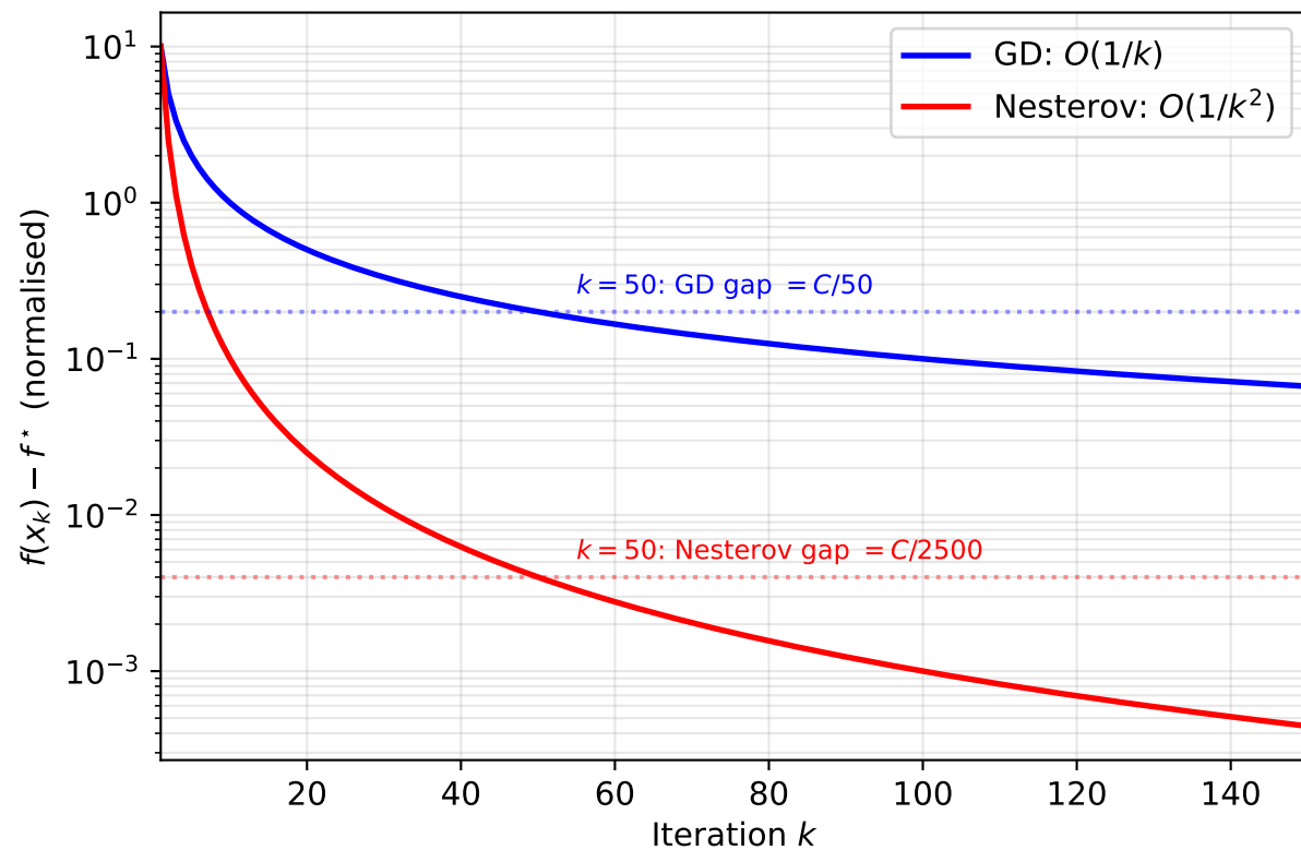
Theoretical Rates: O(1/k) vs O(1/k^2)
