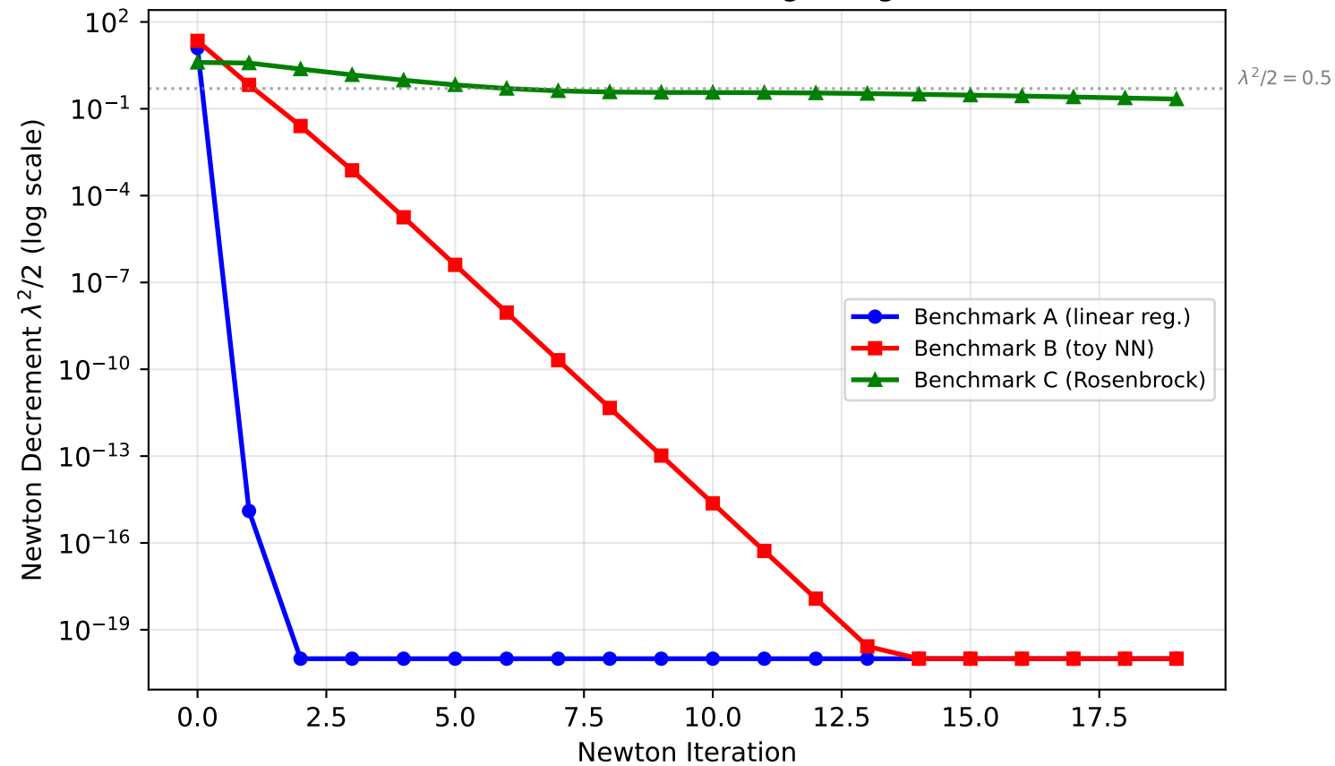
Q3: Newton Decrement \lambda(x)^2/2 = g^T H^{-1} g/2 vs Iteration
