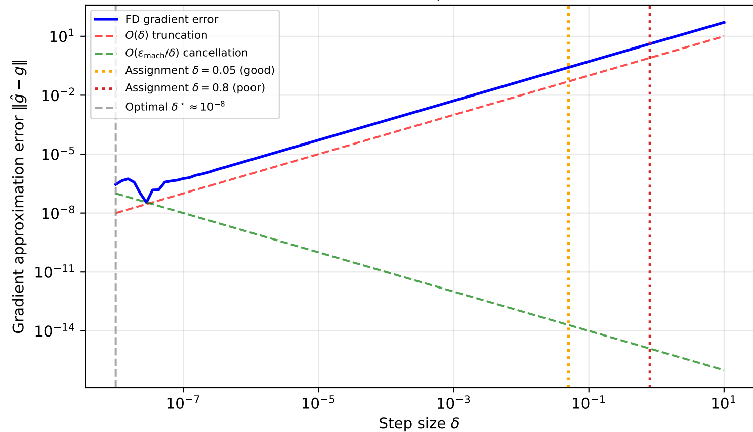
Q4: Forward Finite Difference Error vs Step Size \delta (Benchmark B at x_0 = (-1, 4) )
