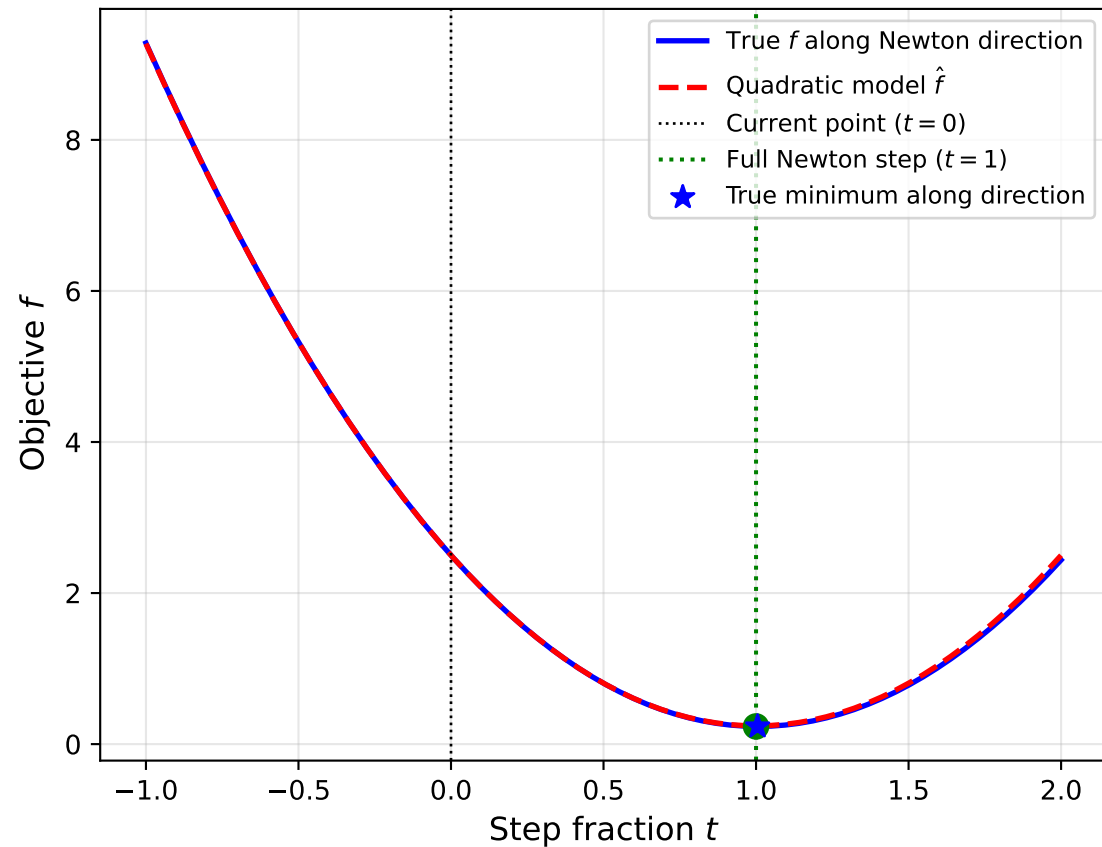
True vs quadratic model at x_0 = (0.5, 0.1)
