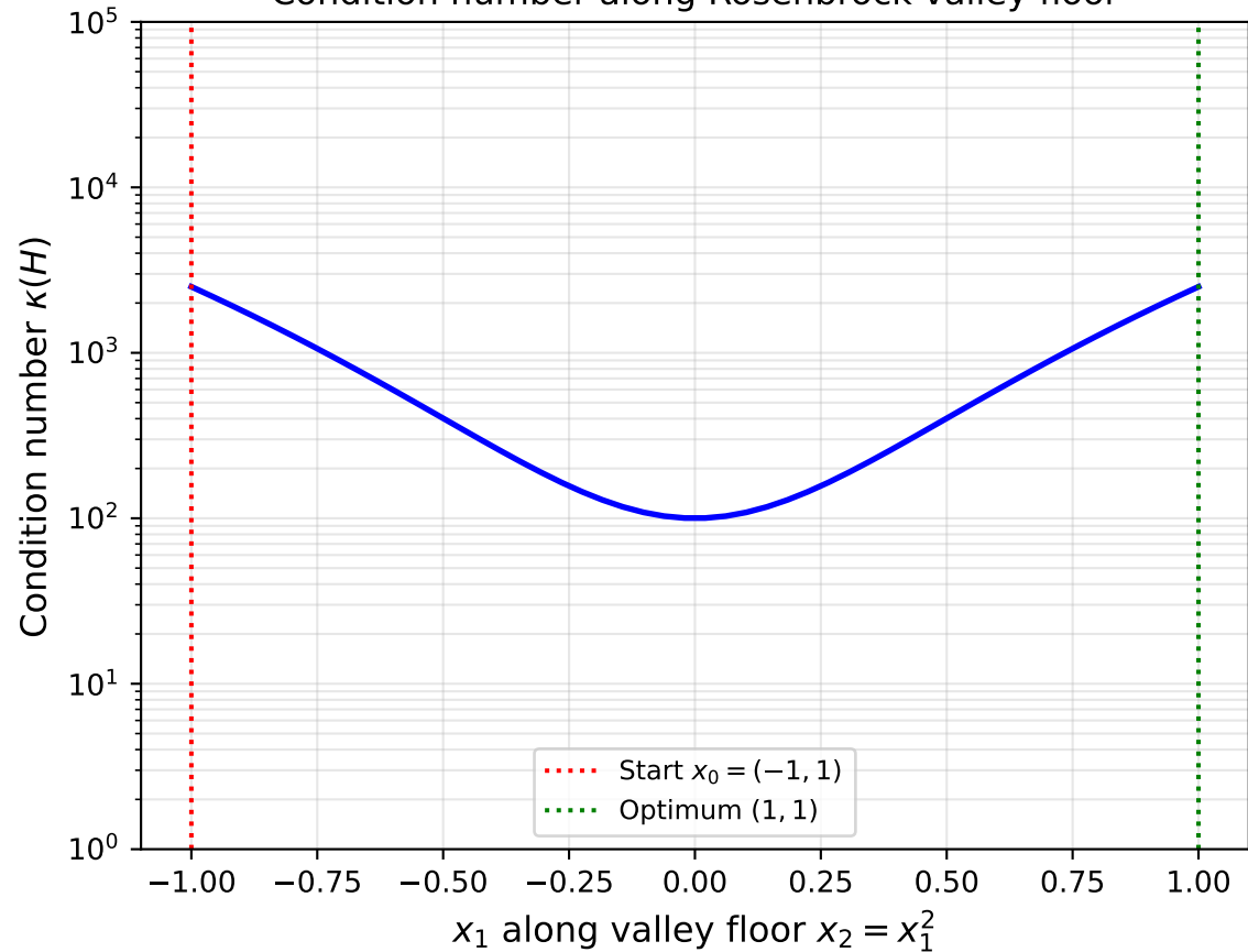
Condition number along Rosenbrock valley floor
