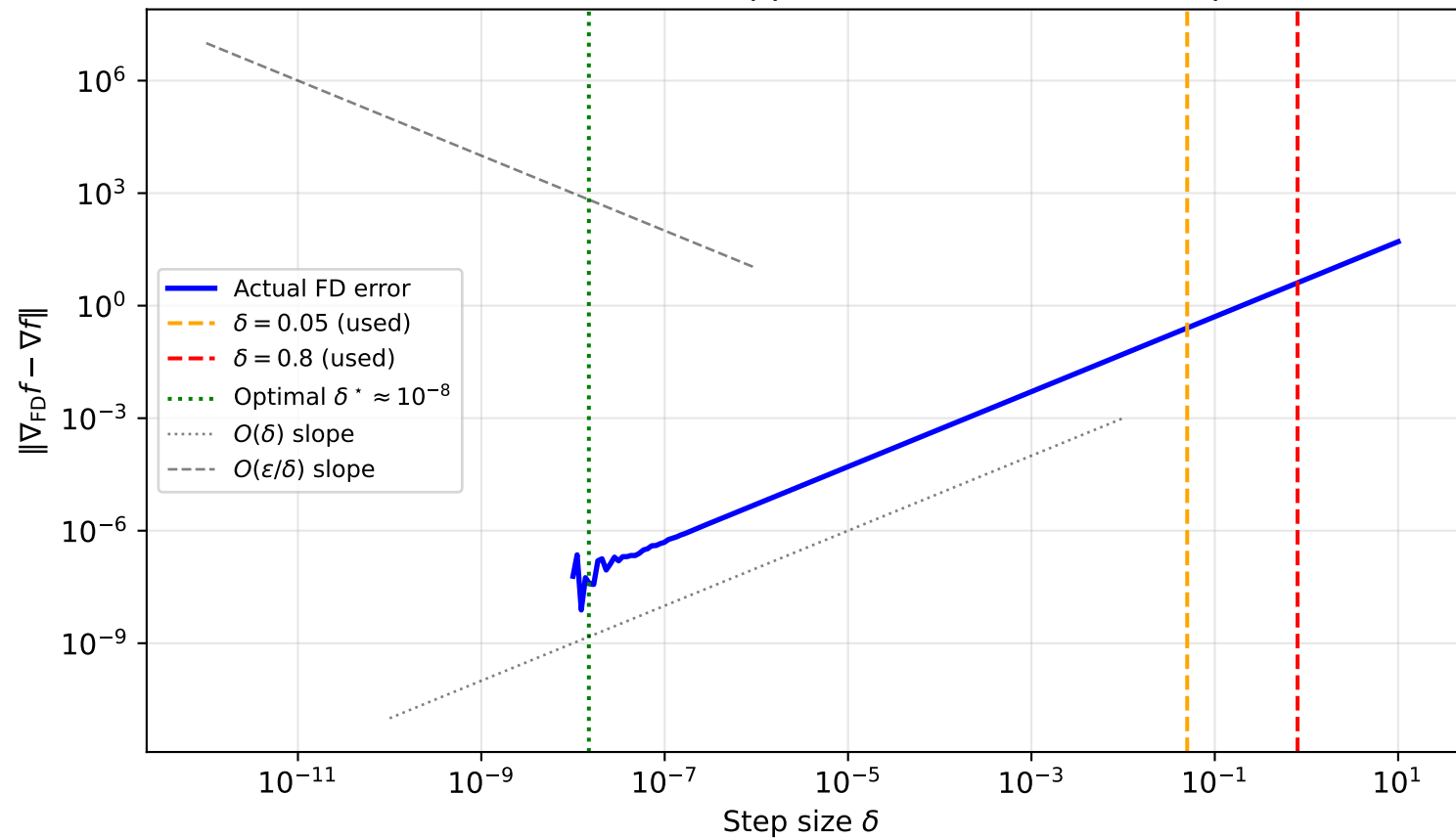
Q4: Forward FD Gradient Approximation Error vs. Step Size
