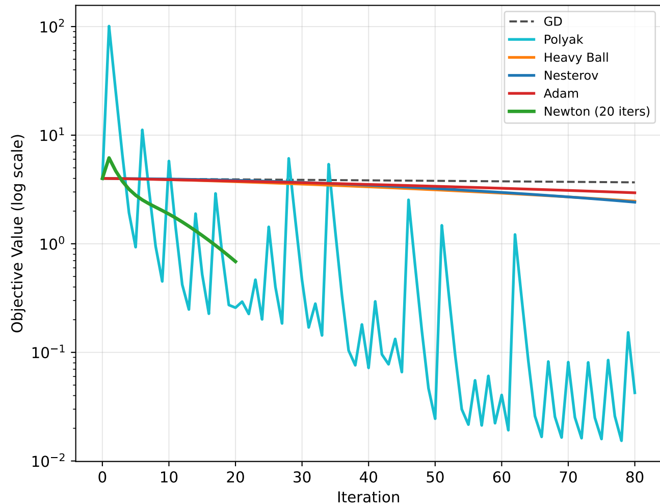
First 80 Iterations (Newton shown for 20)
