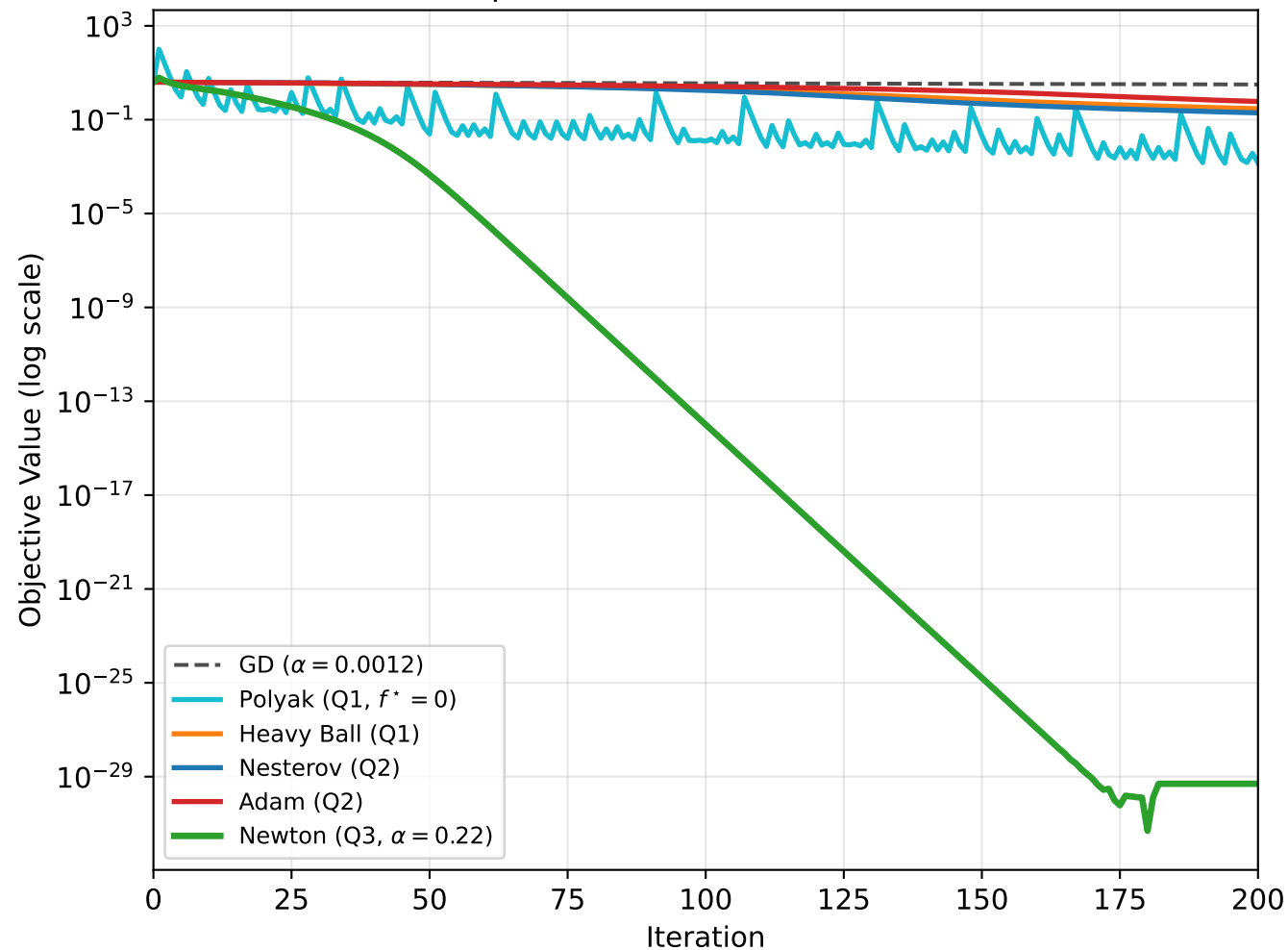
Method Comparison — Rosenbrock (Benchmark C)
