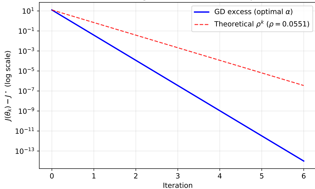
GD Linear Convergence — Benchmark A (optimal \alpha )
