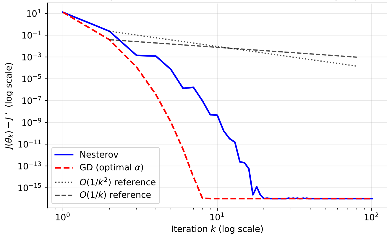
Convergence Rate Verification — Benchmark A (log-log)
