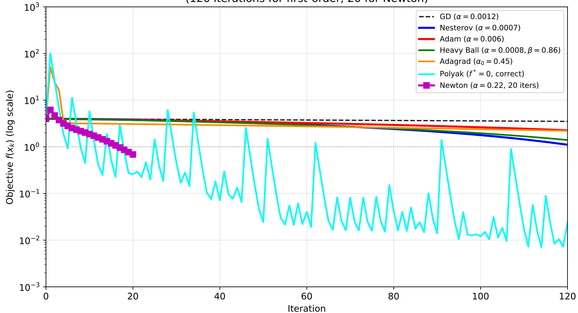
Rosenbrock Benchmark ( \kappa \approx 2504 ): All Methods Summary (120 iterations for first-order, 20 for Newton)
