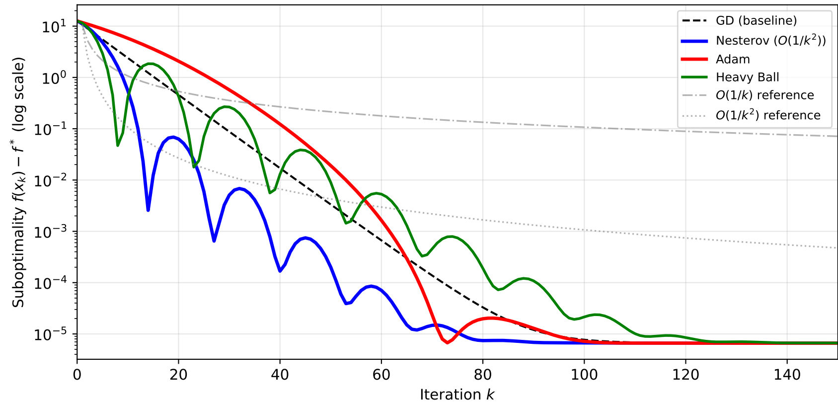
Benchmark A: Convergence Rate Comparison (excess loss above noise floor J^* \approx 0.4826 )
