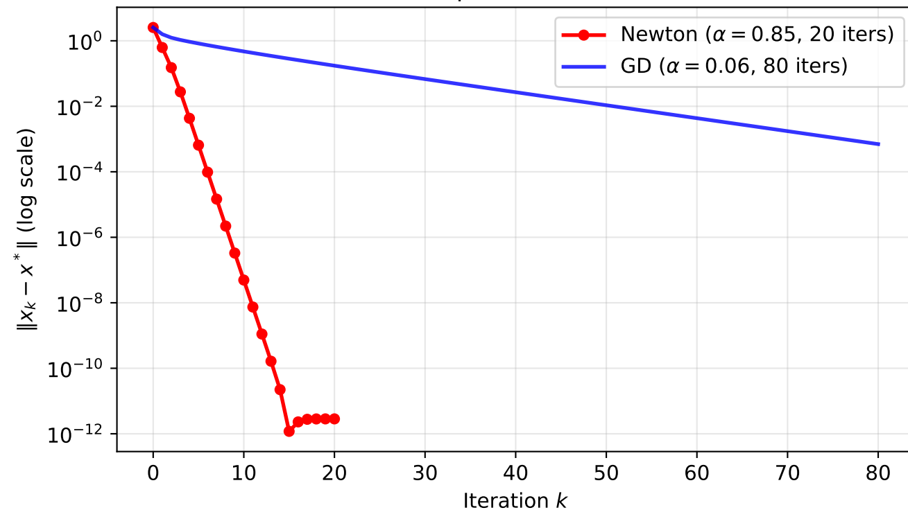
Distance to Optimum (Benchmark B)
