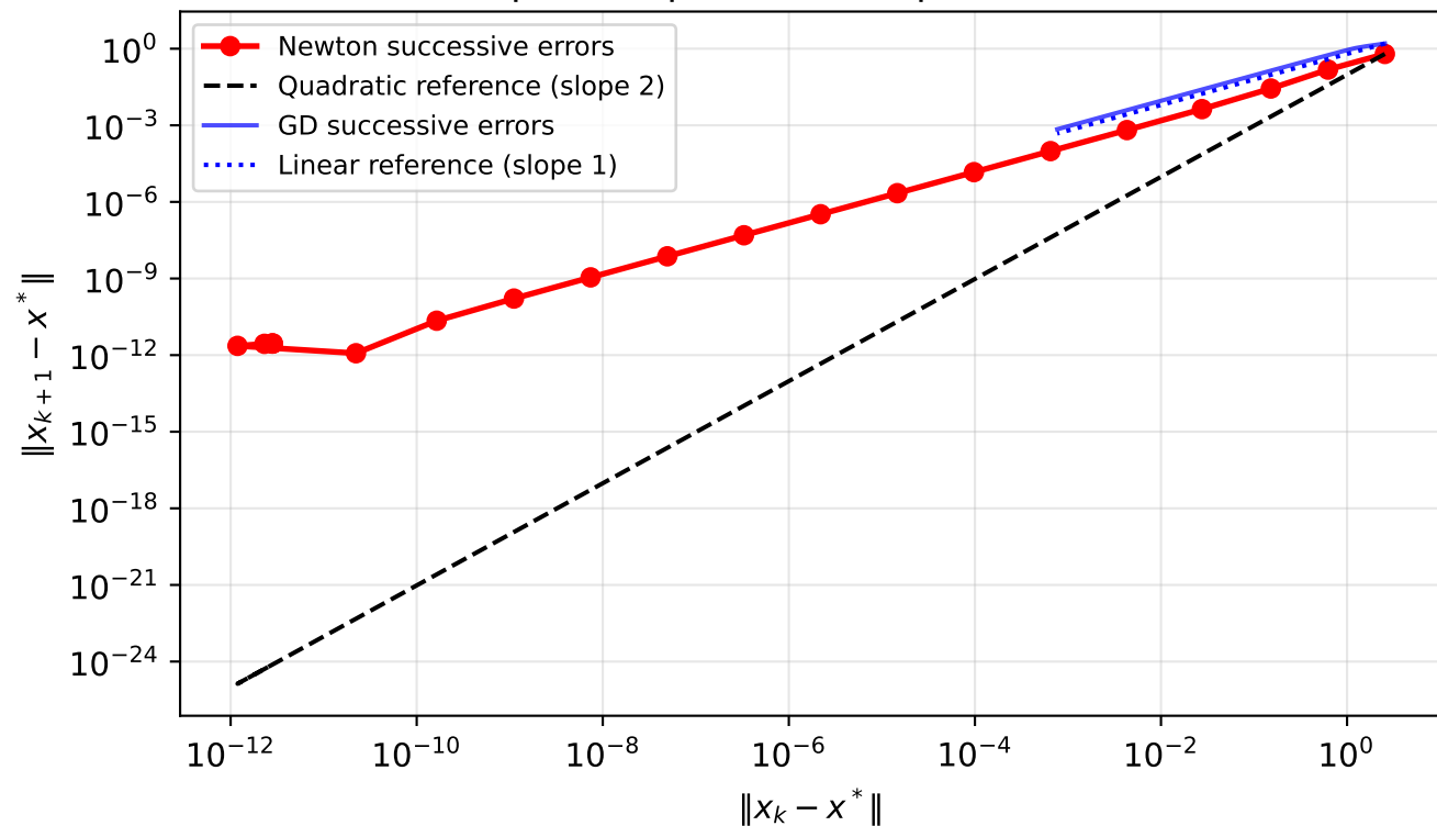
Convergence Order Verification (slope 2 = quadratic, slope 1 = linear)
