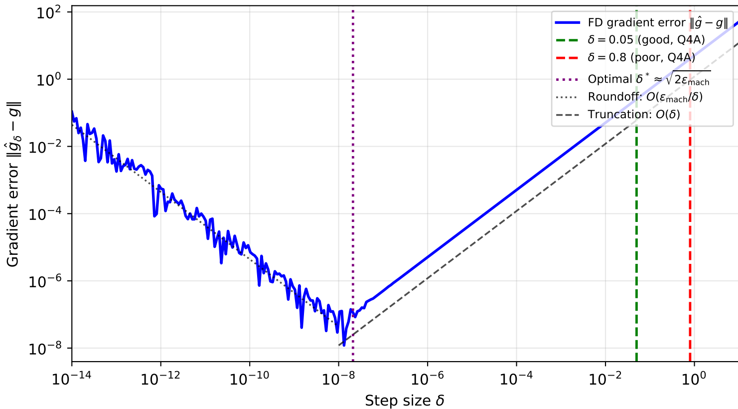
Q4A: Forward FD Gradient Error vs Step Size (Benchmark B, x = (0.3, 2.5) )
