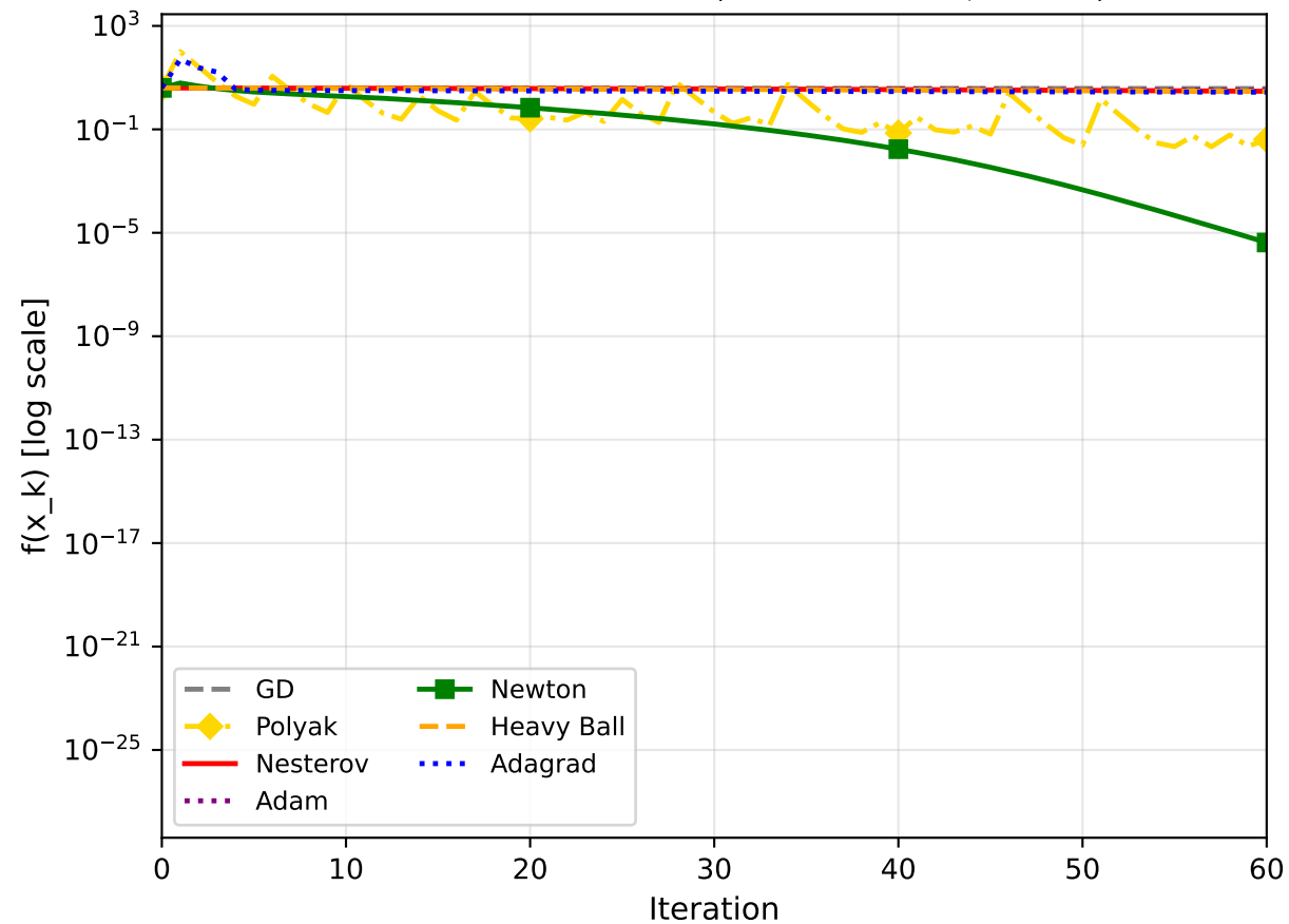
All methods on Rosenbrock (first 60 iterations, zoomed)
