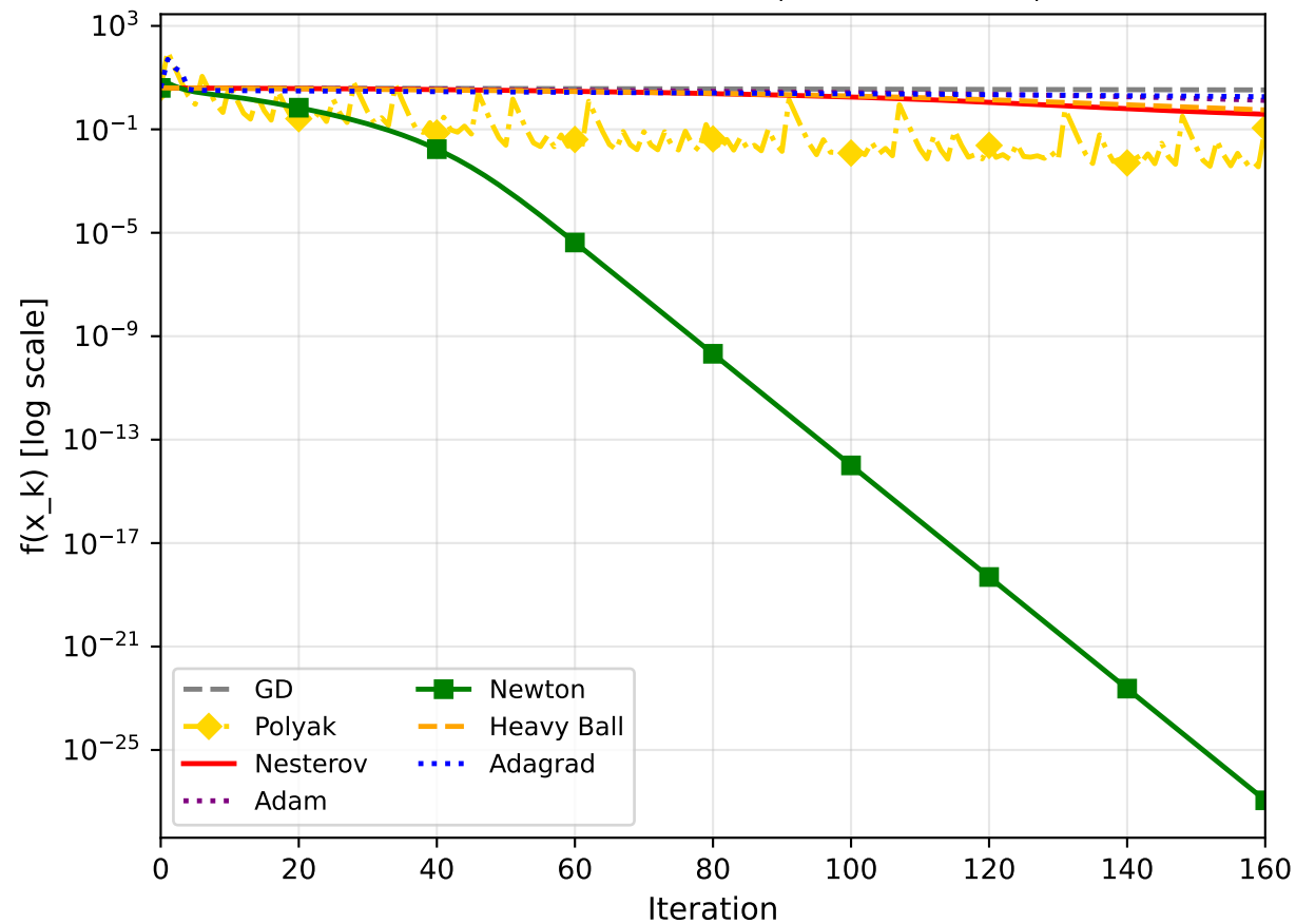
All methods on Rosenbrock (full 160 iterations)
