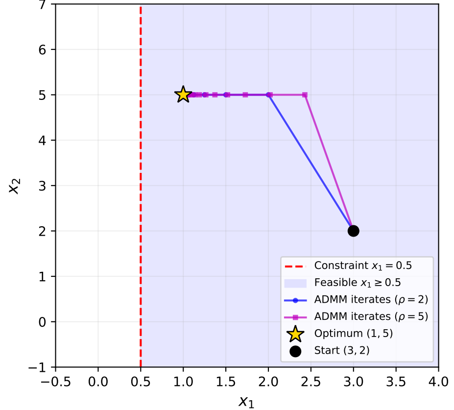
ADMM Iterate Trajectory (constraint x_1 \geq 0.5 shown)
