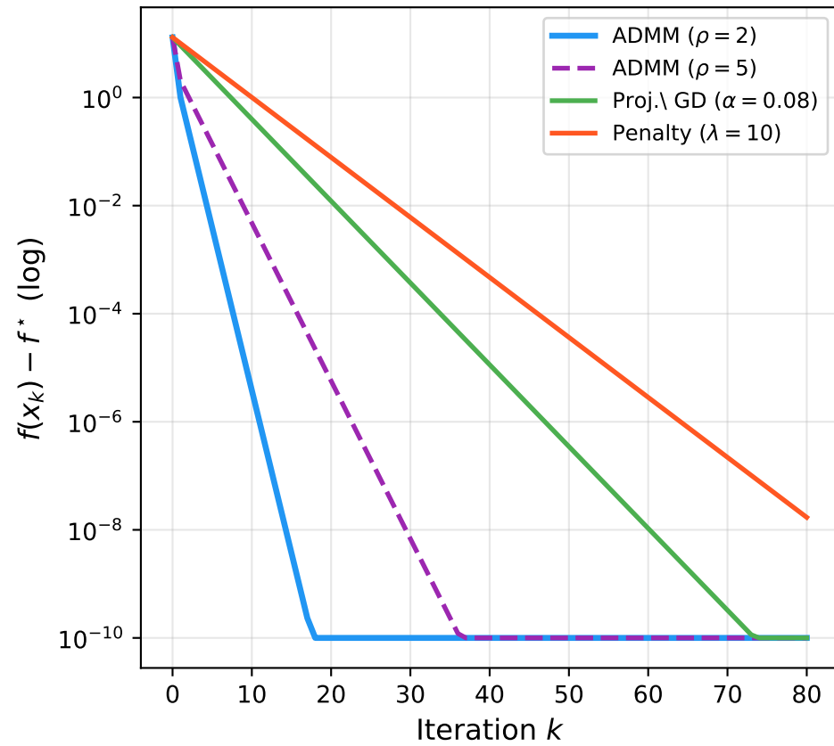
ADMM vs Proj.\ GD vs Penalty (Q5: x_1 \geq 0.5 , starting from (3, 2))
