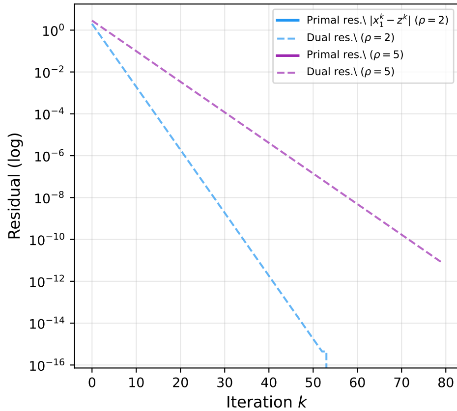
ADMM Primal and Dual Residuals (Convergence certificate)
