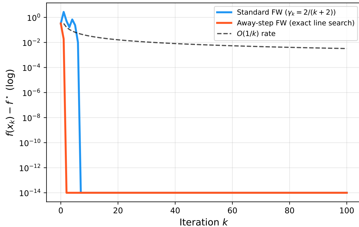
Standard FW vs Away-step FW (Strongly convex quadratic on simplex \Delta^5 )
