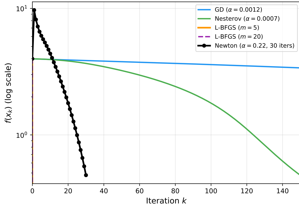
L-BFGS vs Newton vs GD on Rosenbrock (starting from (-1, 1) )
