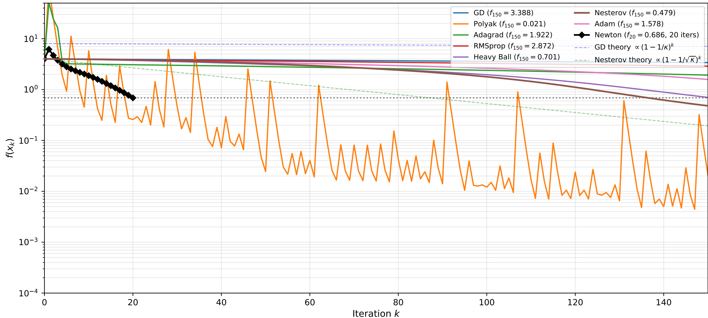
All Methods Convergence on Benchmark C (Rosenbrock, \kappa \approx 2500 ) Semi-log scale: linear convergence appears as straight line; accelerated methods converge faster
