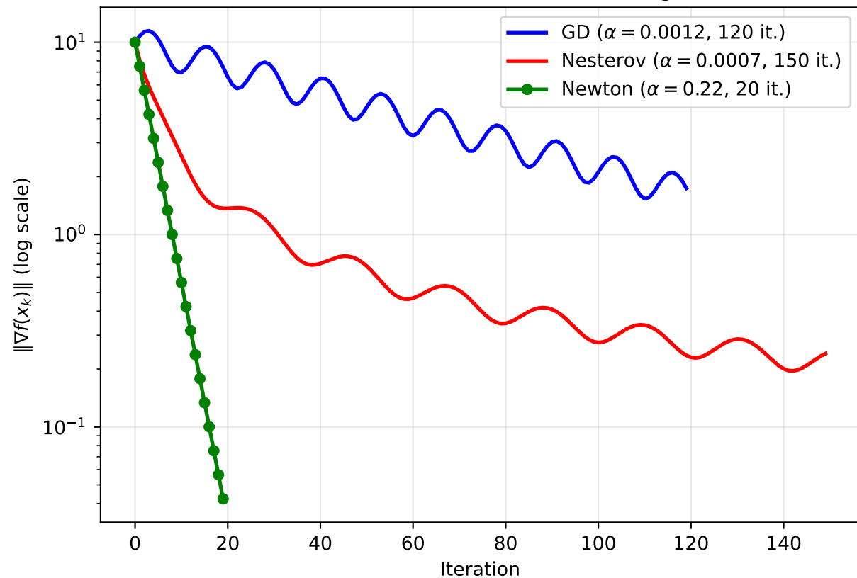
Benchmark C: Gradient Norm vs Iteration (Schematic based on observed convergence)
