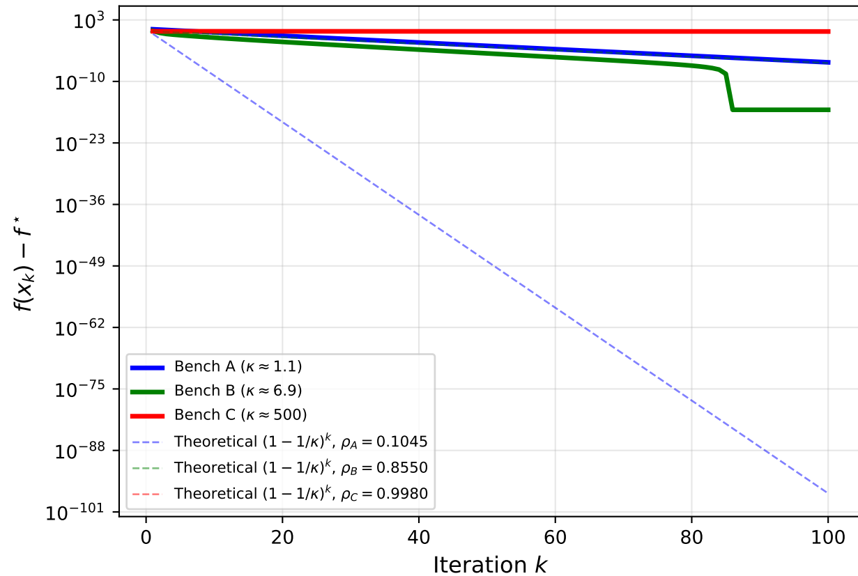
GD convergence across benchmarks (theoretical vs empirical rates)
