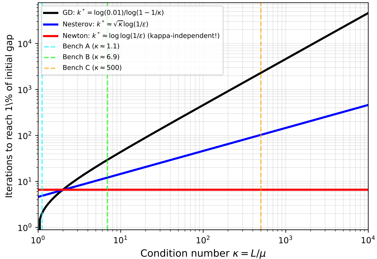
Iterations to convergence vs. condition number (GD, Nesterov, Newton)
