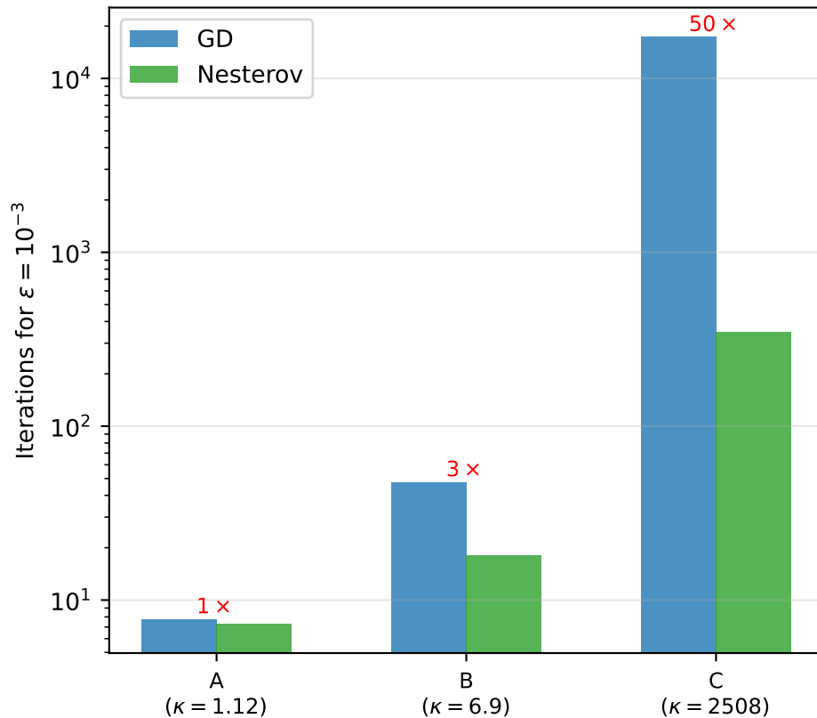
Required Iterations at \varepsilon = 10^{-3} (theoretical \kappa \log(1/\varepsilon) bound)
