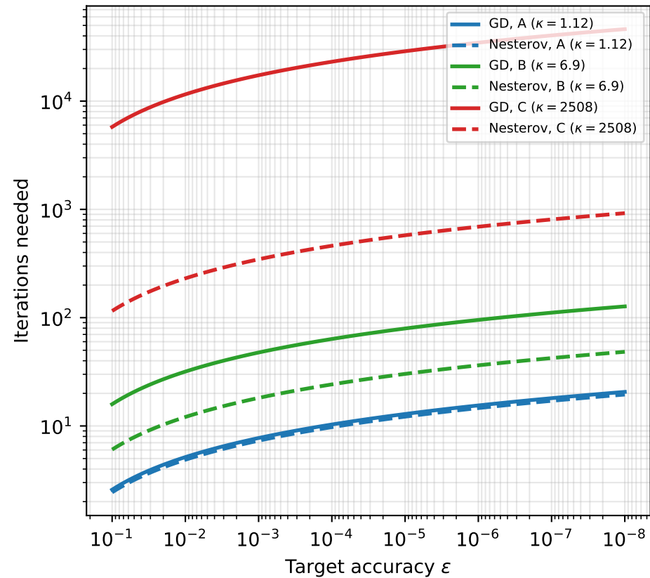
Oracle Complexity (strongly convex)
