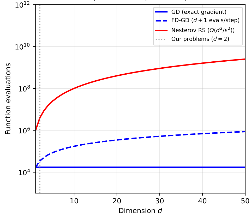
Scaling with Dimension (Rosenbrock, \varepsilon = 10^{-3} )
