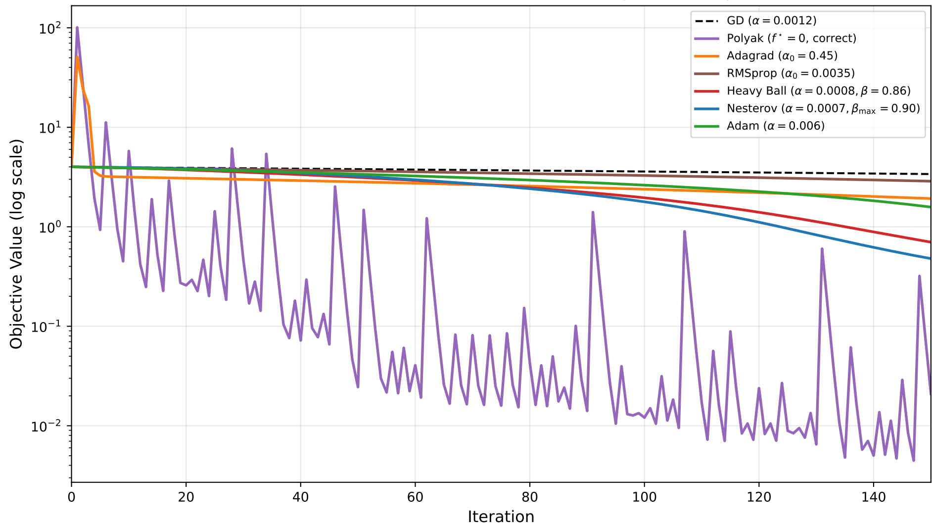
All First-Order Methods on Benchmark C (Rosenbrock)
