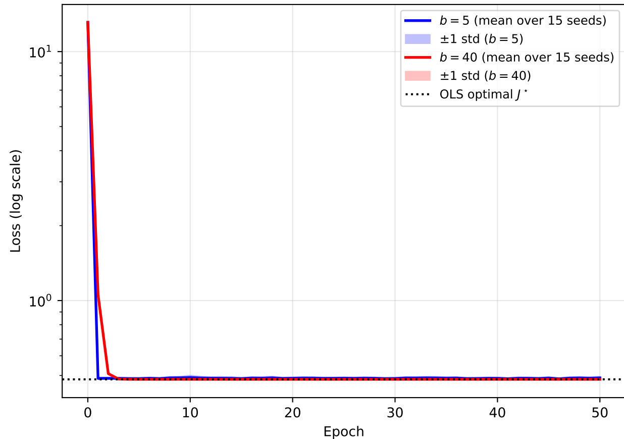
Q2: SGD Mean \pm Std Across 15 Random Seeds
