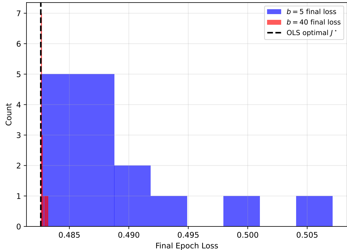
Q2: Distribution of Final Loss Across 15 Seeds
