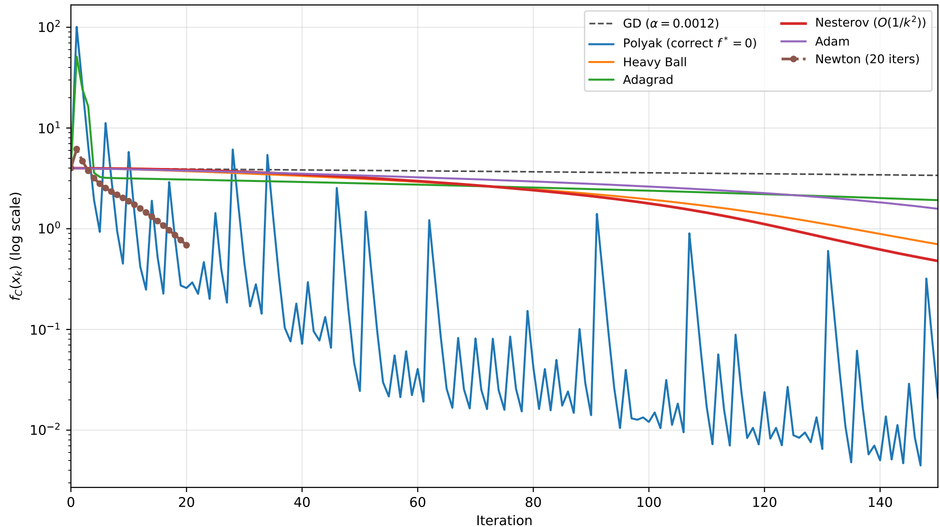
All Methods: Convergence on Rosenbrock ( \kappa \approx 2508 )
