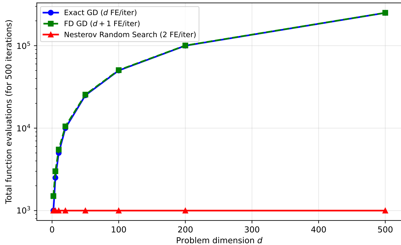
Q4: Scaling of Function Evaluation Cost with Dimension
