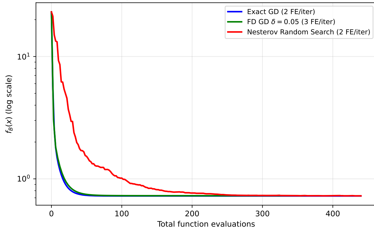
Q4: Convergence vs Function Evaluations — Benchmark B
