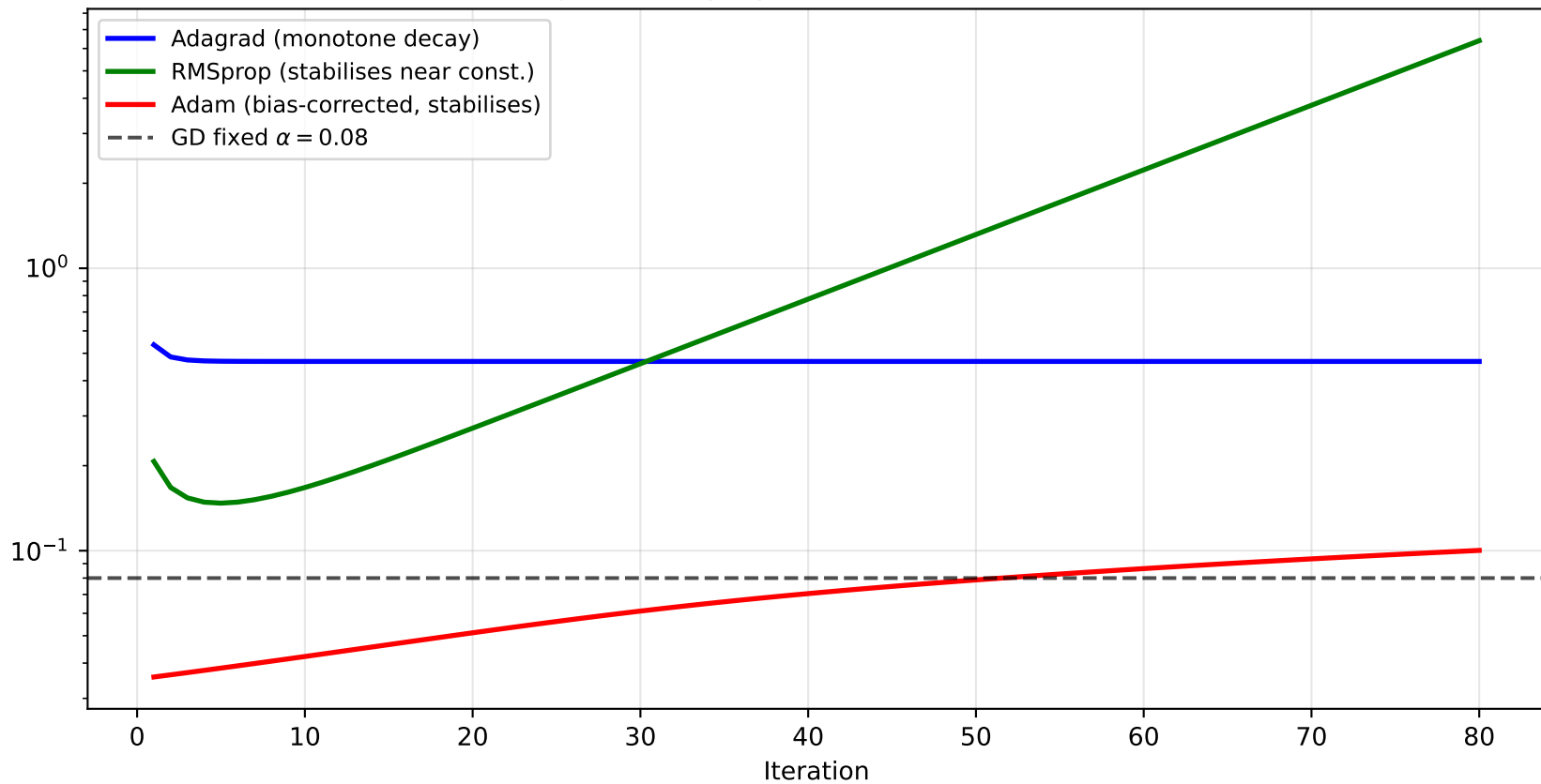
Q1/Q2: Effective Learning Rate Comparison (Adagrad, RMSprop, Adam on Benchmark A)
