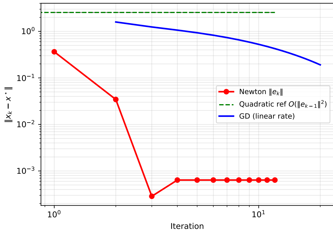
Convergence Rate Verification (log--log) Quadratic vs Linear
