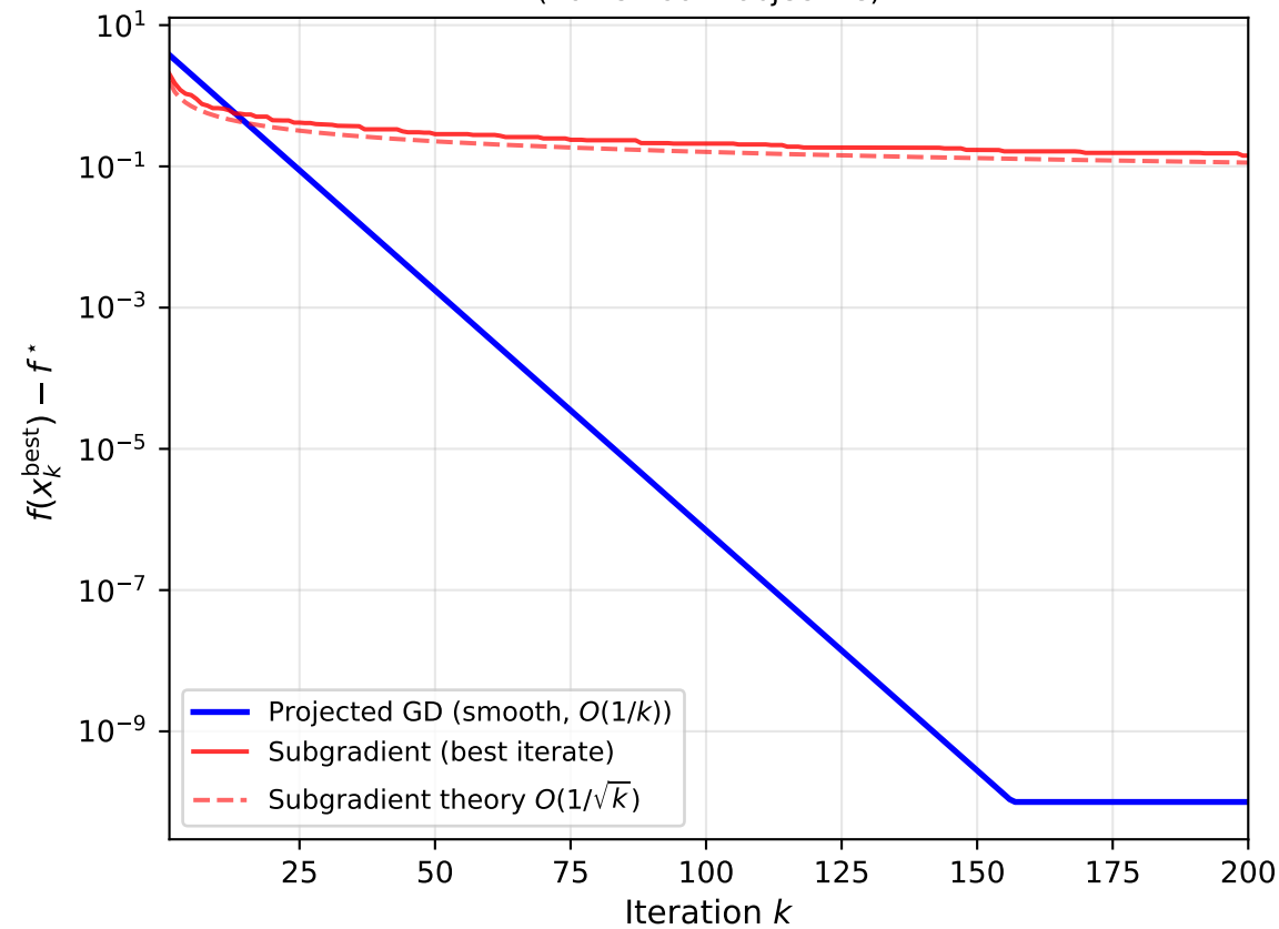
Subgradient vs Projected GD (non-smooth objective)
