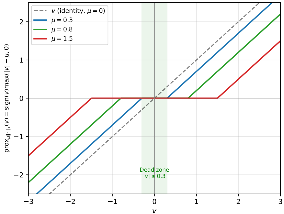
Soft-Thresholding: Proximal Operator of \mu\|\cdot\|_1 (ISTA/FISTA step for Lasso)
