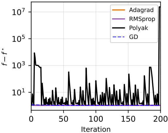
Bench. B: Adaptive Methods
