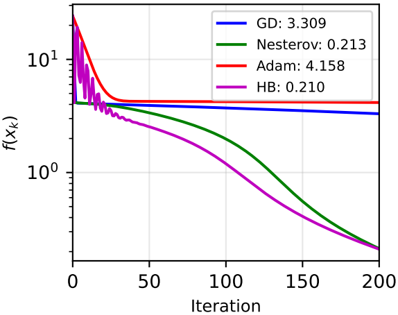
Bench. C: Rosenbrock (Q2)
