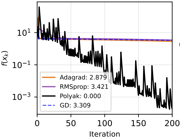
Bench. C: Rosenbrock (Q1)
