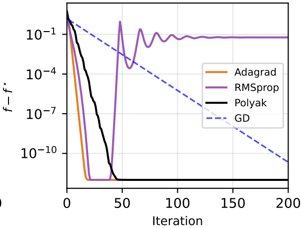
Bench. A: Adaptive Methods
