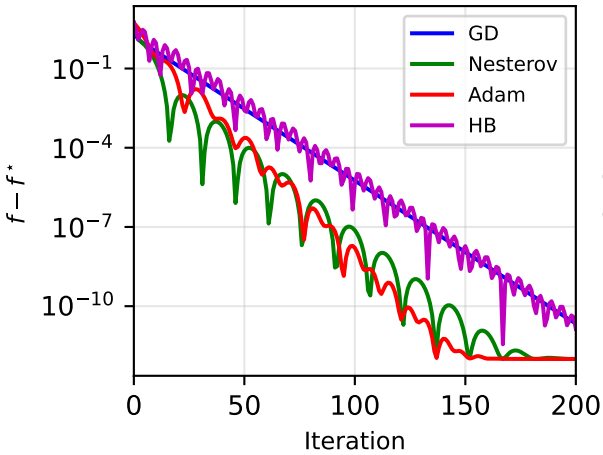
Bench. A: Quadratic
