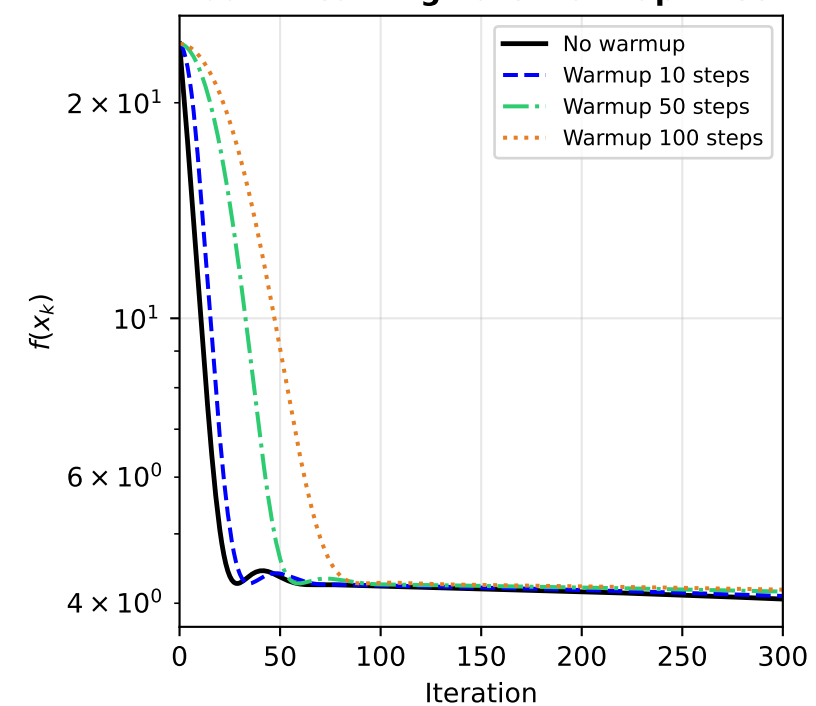
Adam: Learning Rate Warmup Effect
