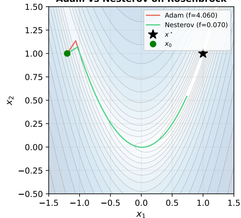
Adam vs Nesterov on Rosenbrock
