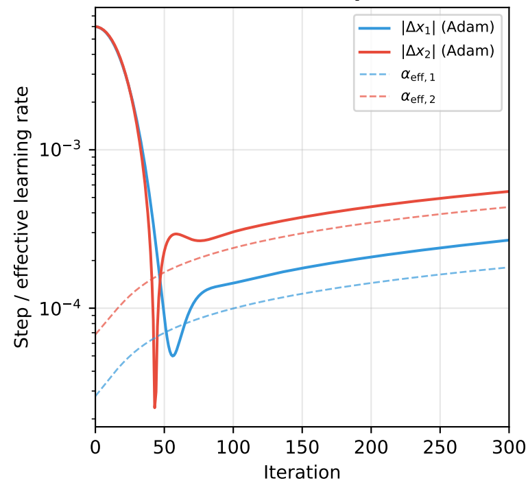
Adam Per-Coordinate Steps (Rosenbrock)
