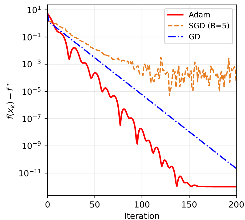
Adam vs SGD vs GD: Benchmark A
