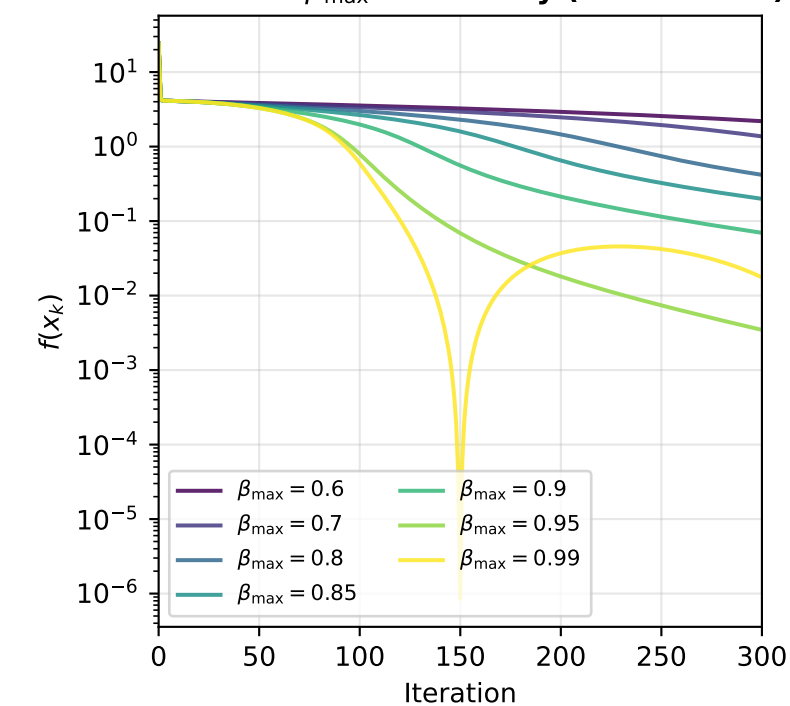
Nesterov: \beta_{\text{max}} Sensitivity (Rosenbrock)
