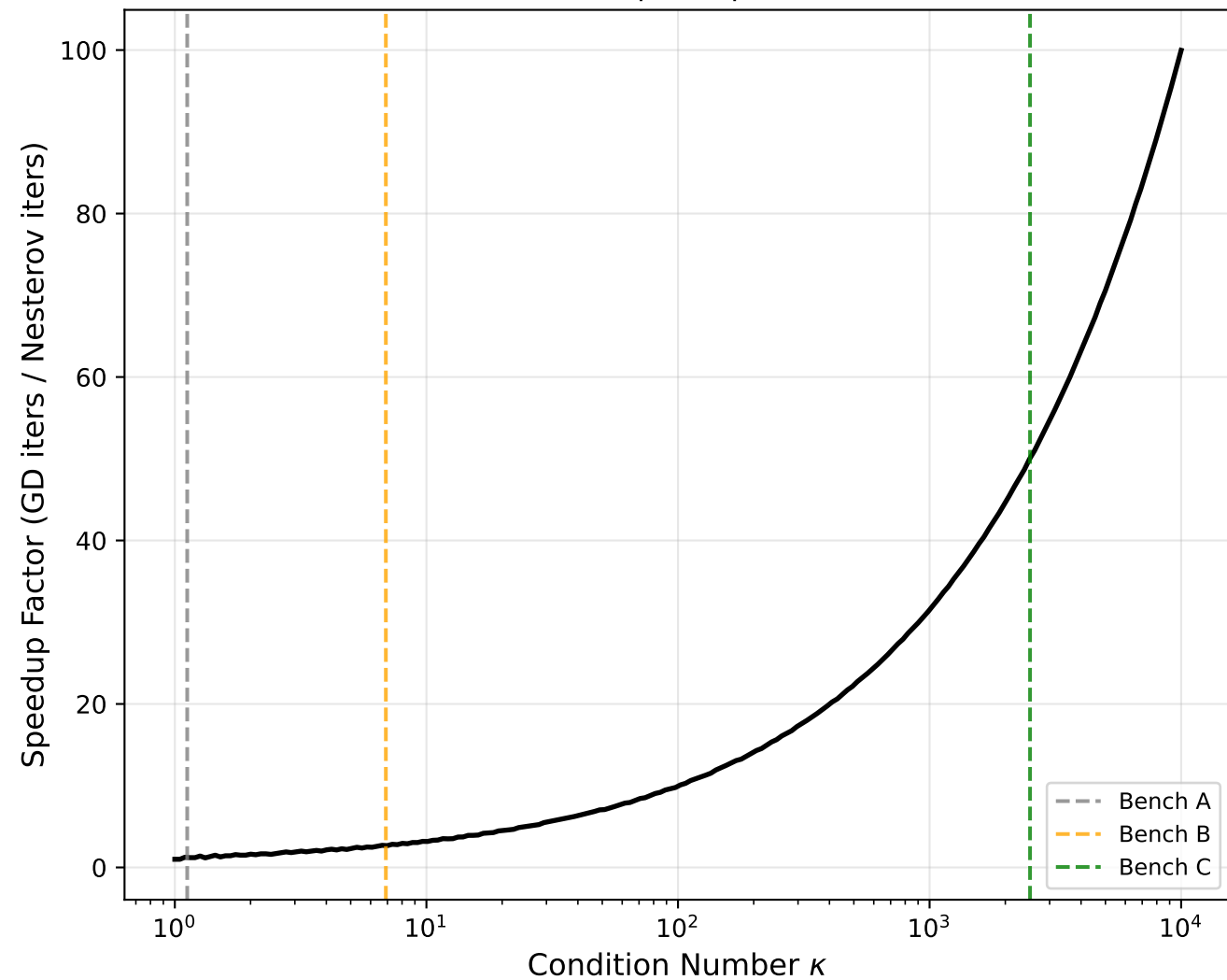
Nesterov Speedup over GD
