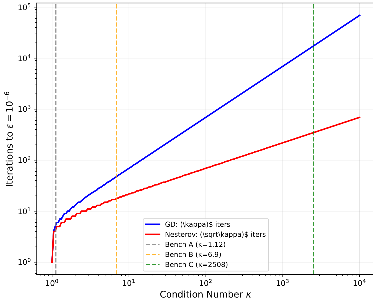
Theoretical Iterations: GD vs Nesterov
