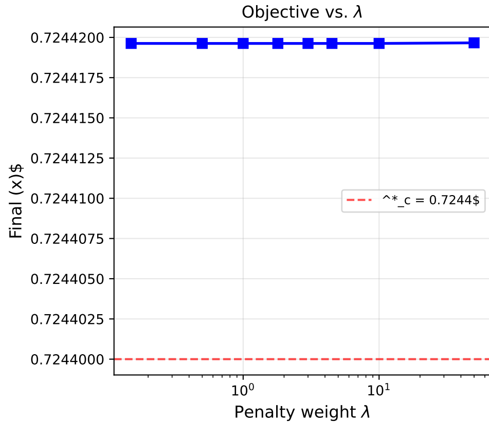
Q5: Penalty Method --- Effect of \lambda (200 iters, \alpha = 0.03 )
