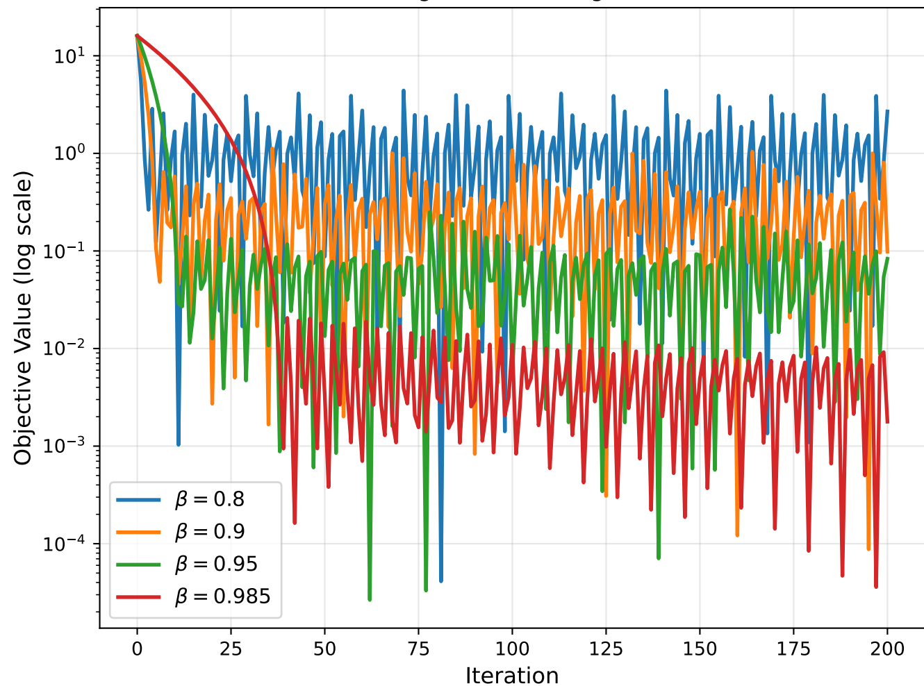
FW Convergence vs. Mixing Parameter
