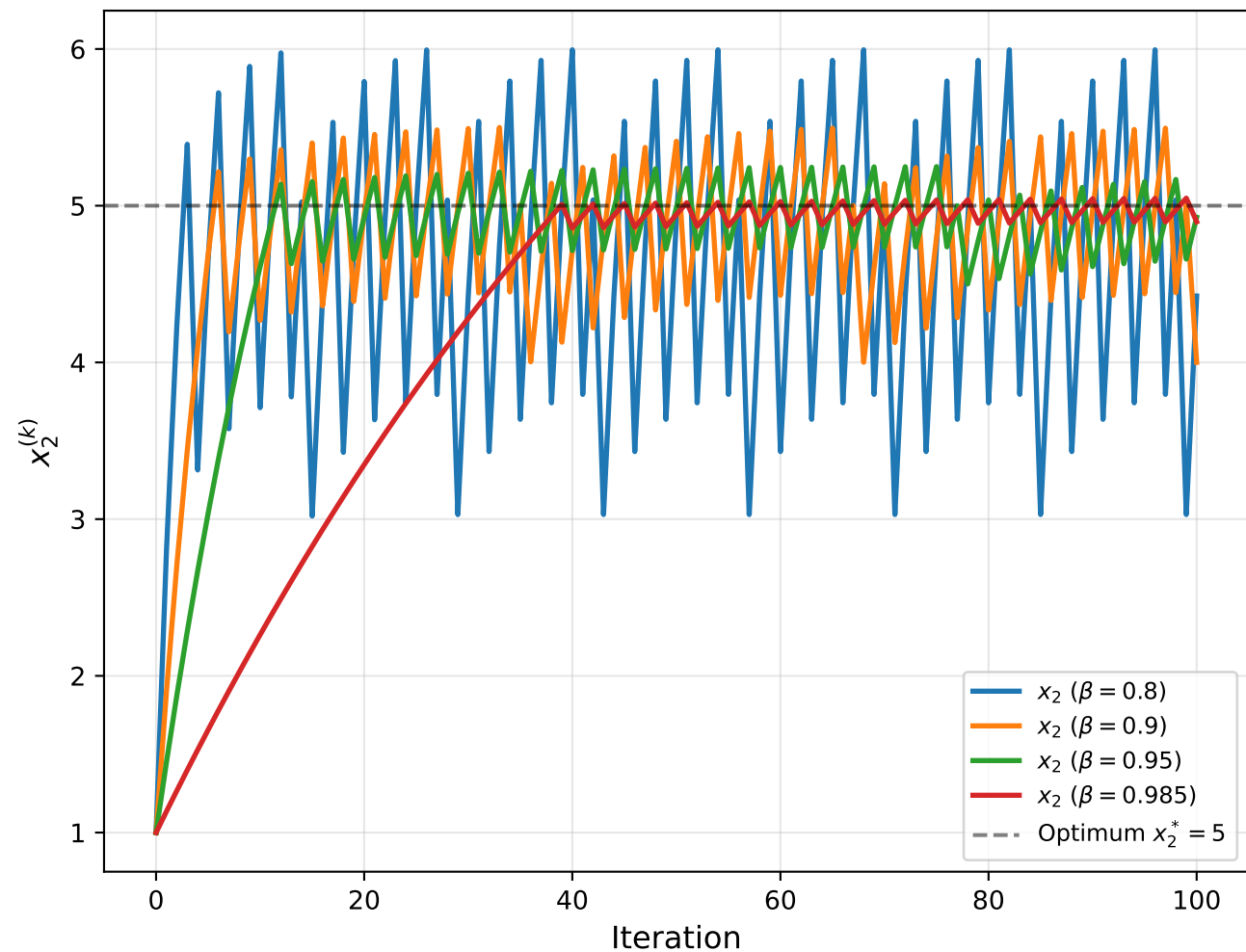
x_2 Component Evolution
