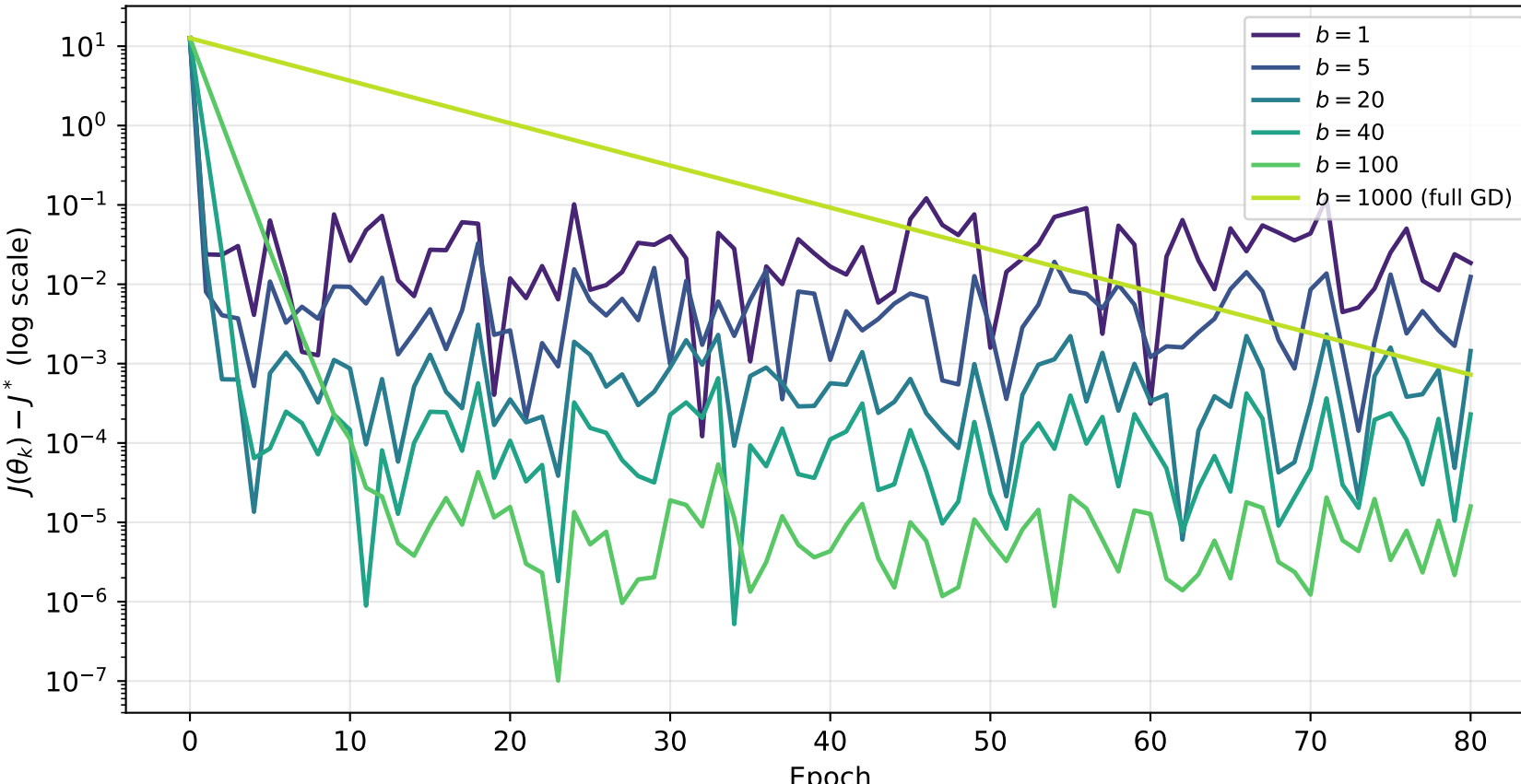
Q2: SGD Suboptimality Gap by Batch Size — Benchmark A (80 epochs)
