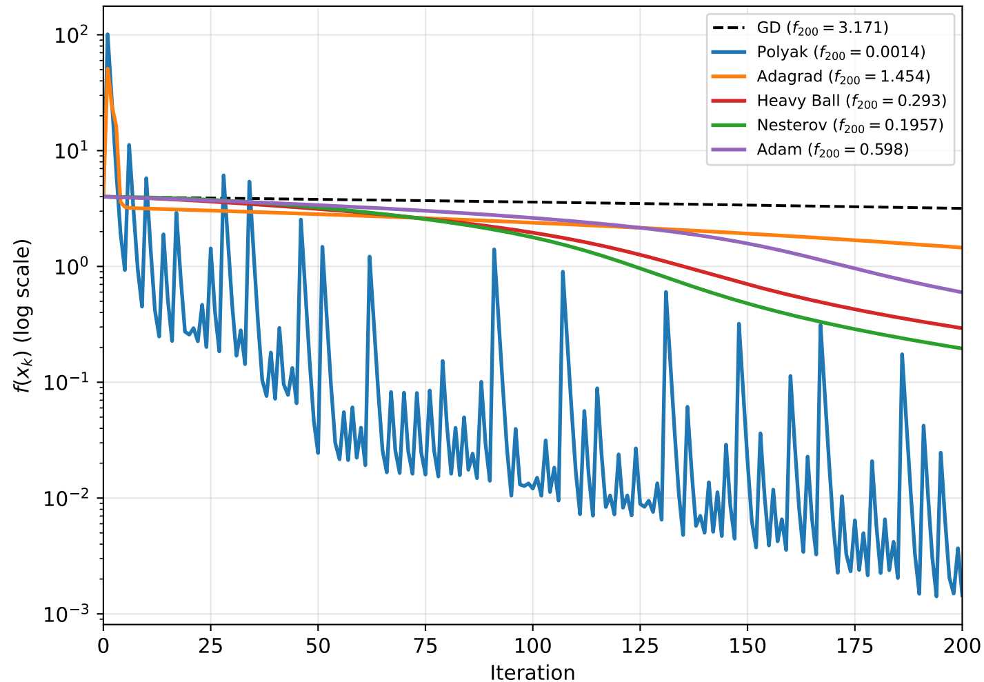
All First-Order Methods — Benchmark C (200 iters)
