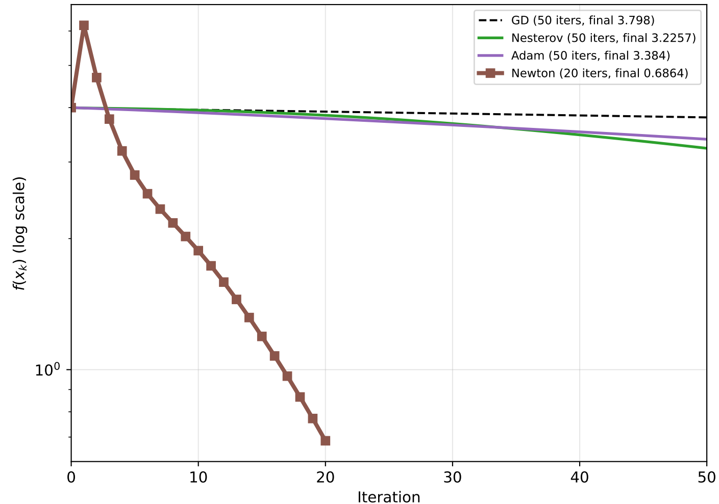
Newton vs Best First-Order — First 50 Iters
