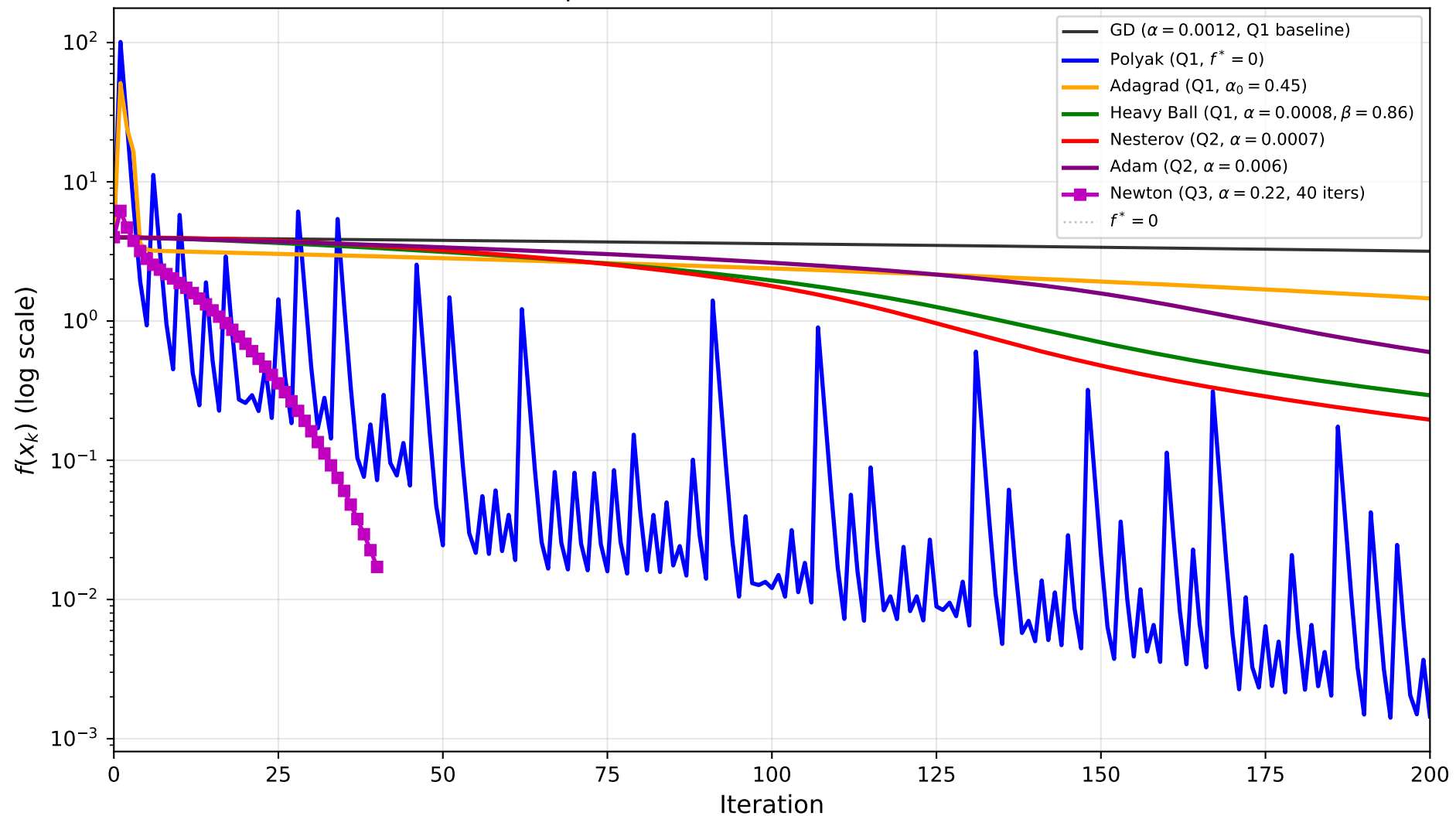
Cross-Question Comparison: All Methods on Benchmark C (Rosenbrock)
