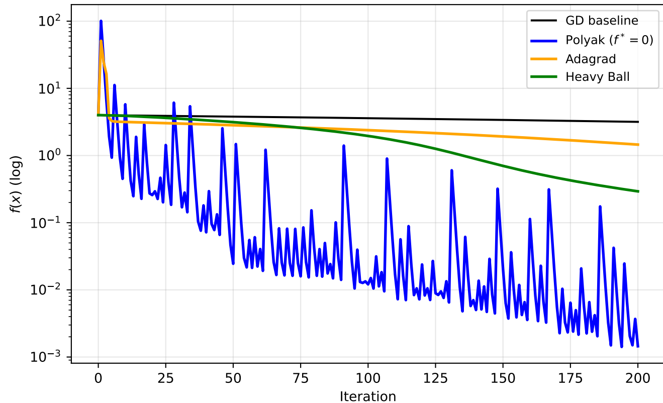
Q1 Adaptive Methods on Rosenbrock
