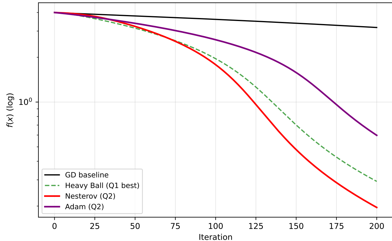
Q2 Momentum Methods on Rosenbrock
