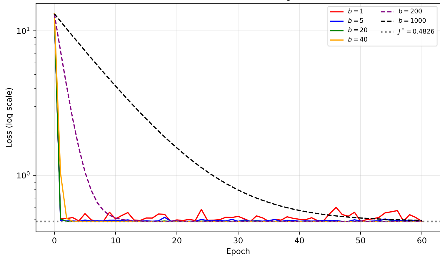
Mini-Batch SGD: Effect of Batch Size on Convergence Rate (Benchmark A)
