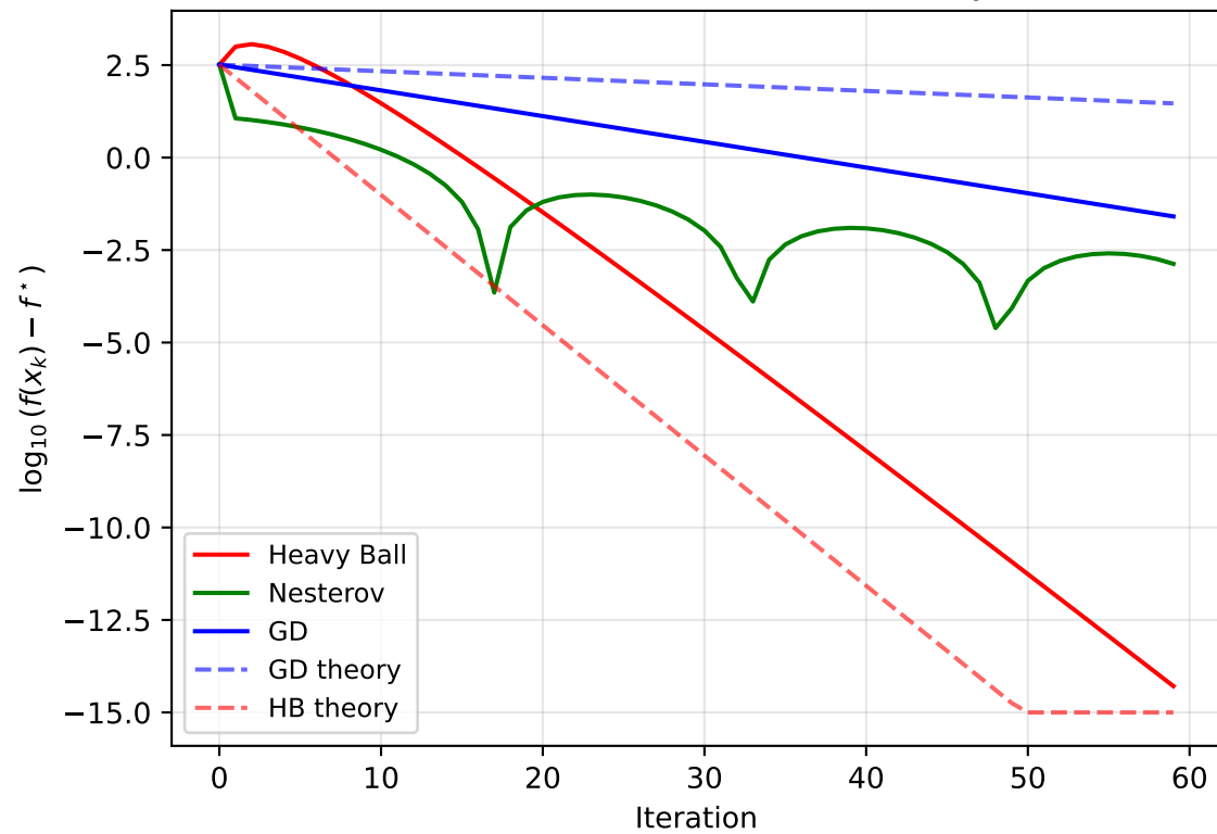
First 60 iterations: oscillation in Heavy Ball
