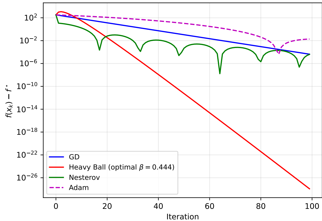
Convergence on quadratic ( \kappa = 25.0 )
