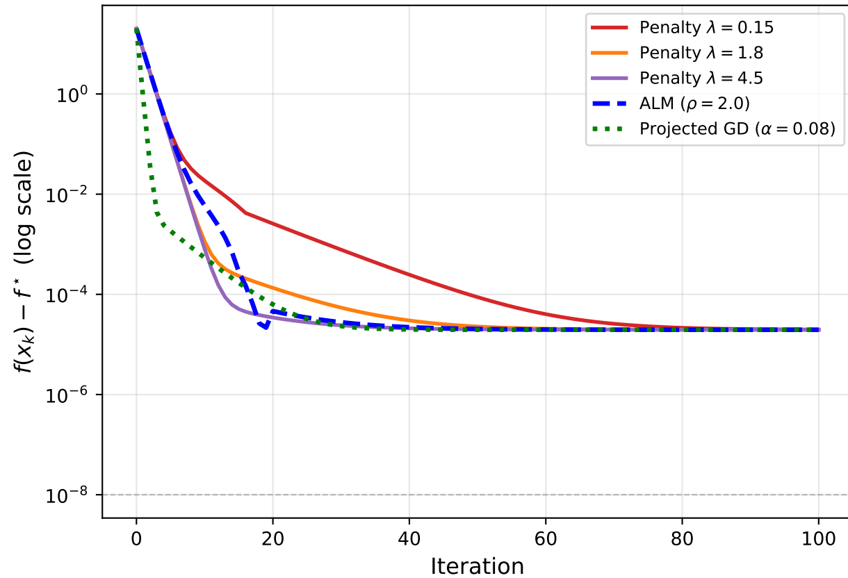
Objective Convergence: Penalty vs ALM vs Projected GD
