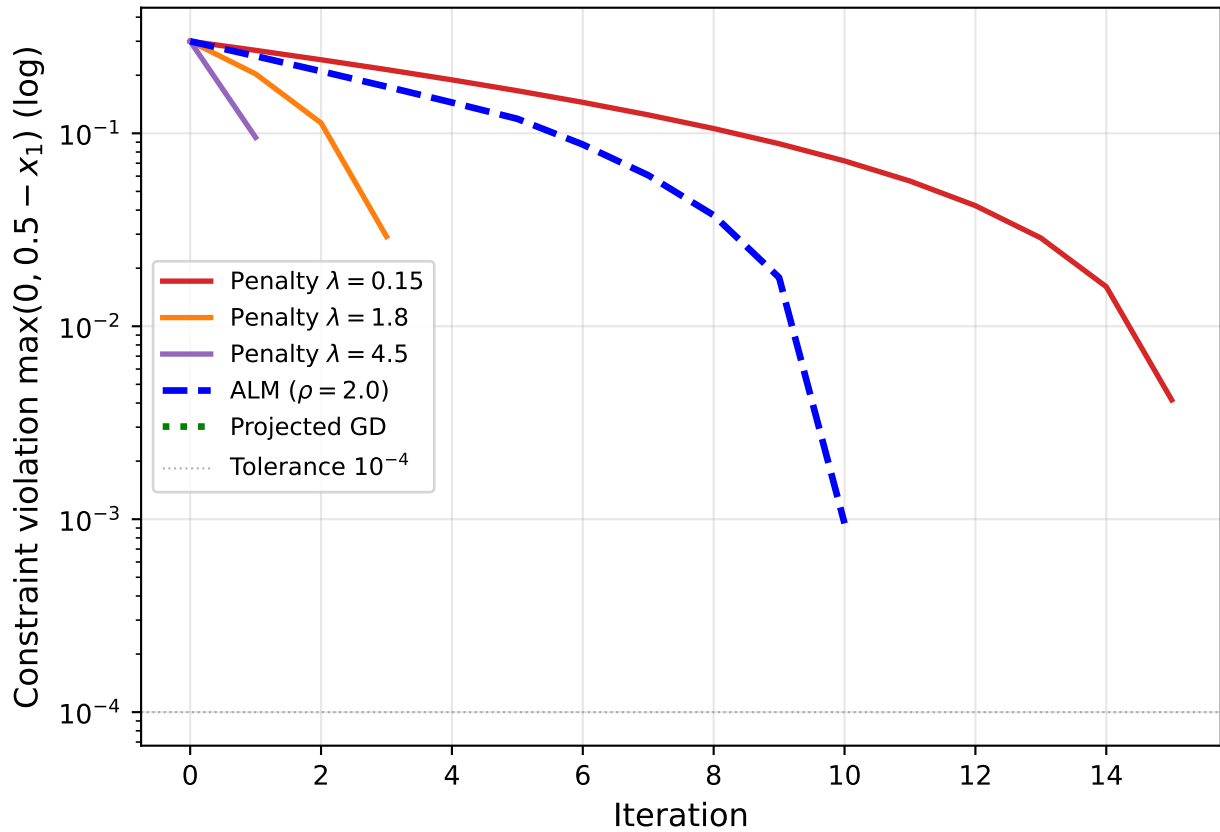
Constraint Violation: Penalty vs ALM vs Projected GD
