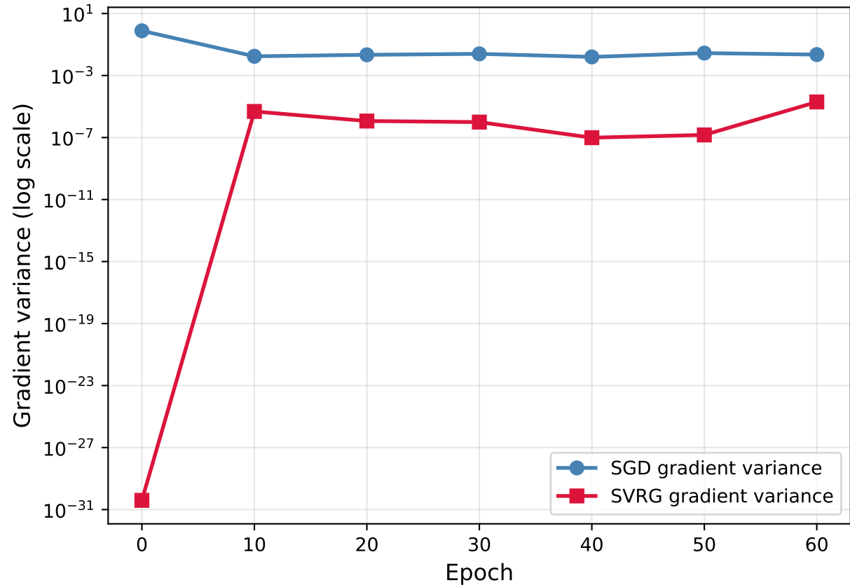
Gradient Variance: SGD vs SVRG (Benchmark A, b=40 )
