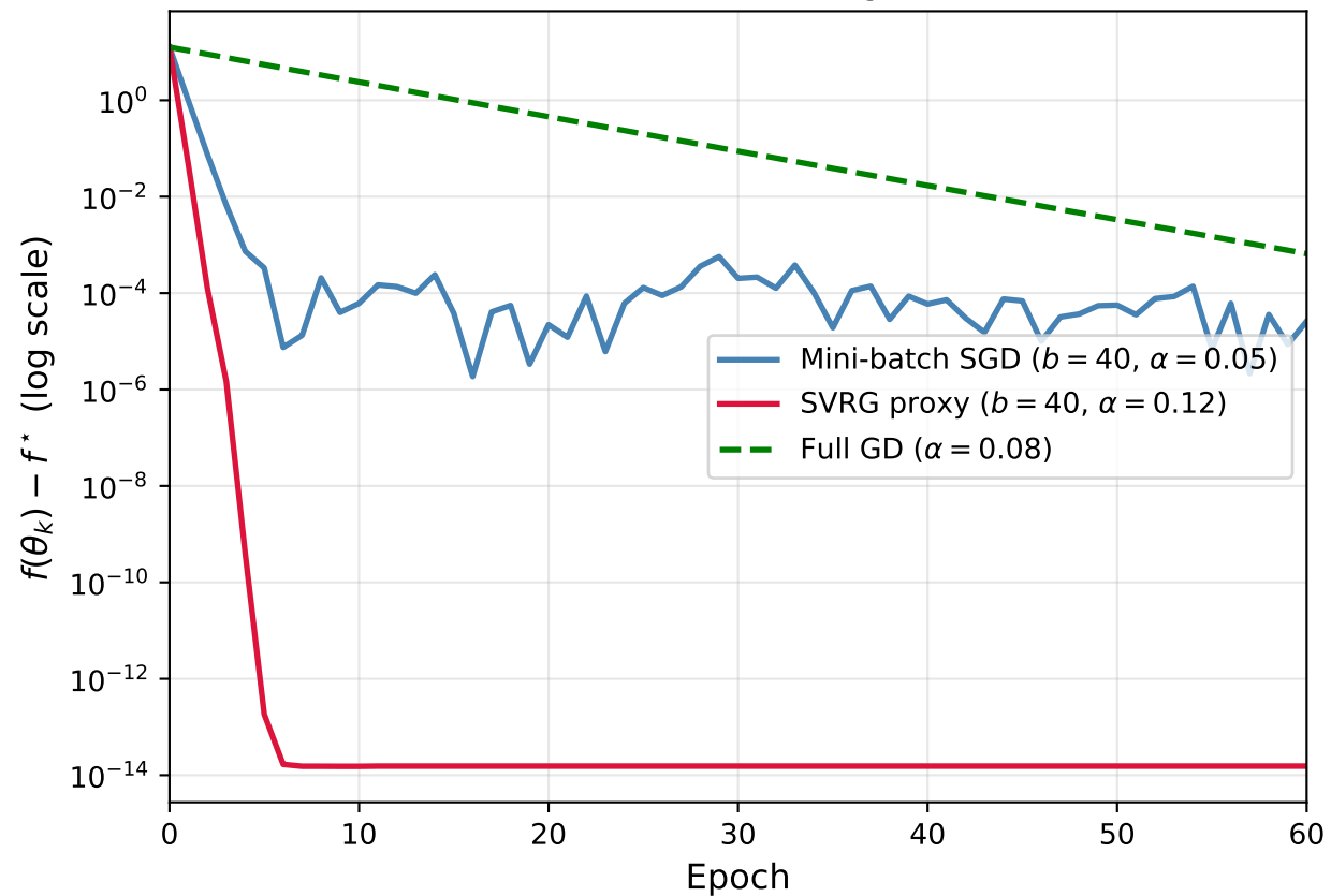
SGD vs Variance-Reduced SGD (SVRG) Benchmark A: Linear Regression
