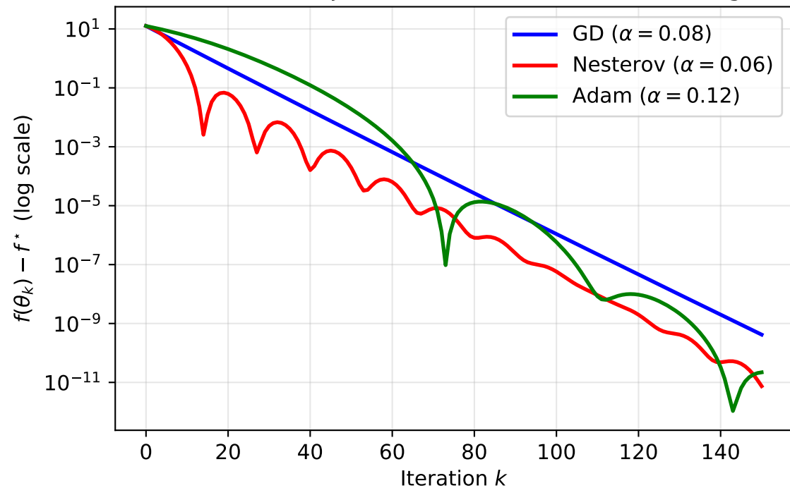
Q2: Excess Objective on Benchmark A (semilog)
