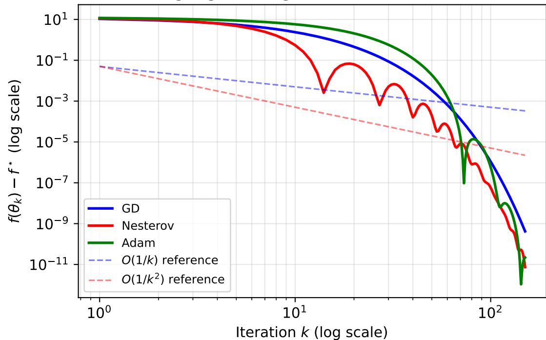
Q2: Log-log convergence (rate identification)
