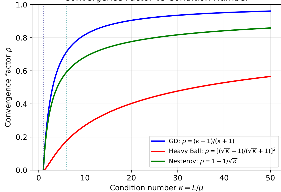
Convergence Factor vs Condition Number
