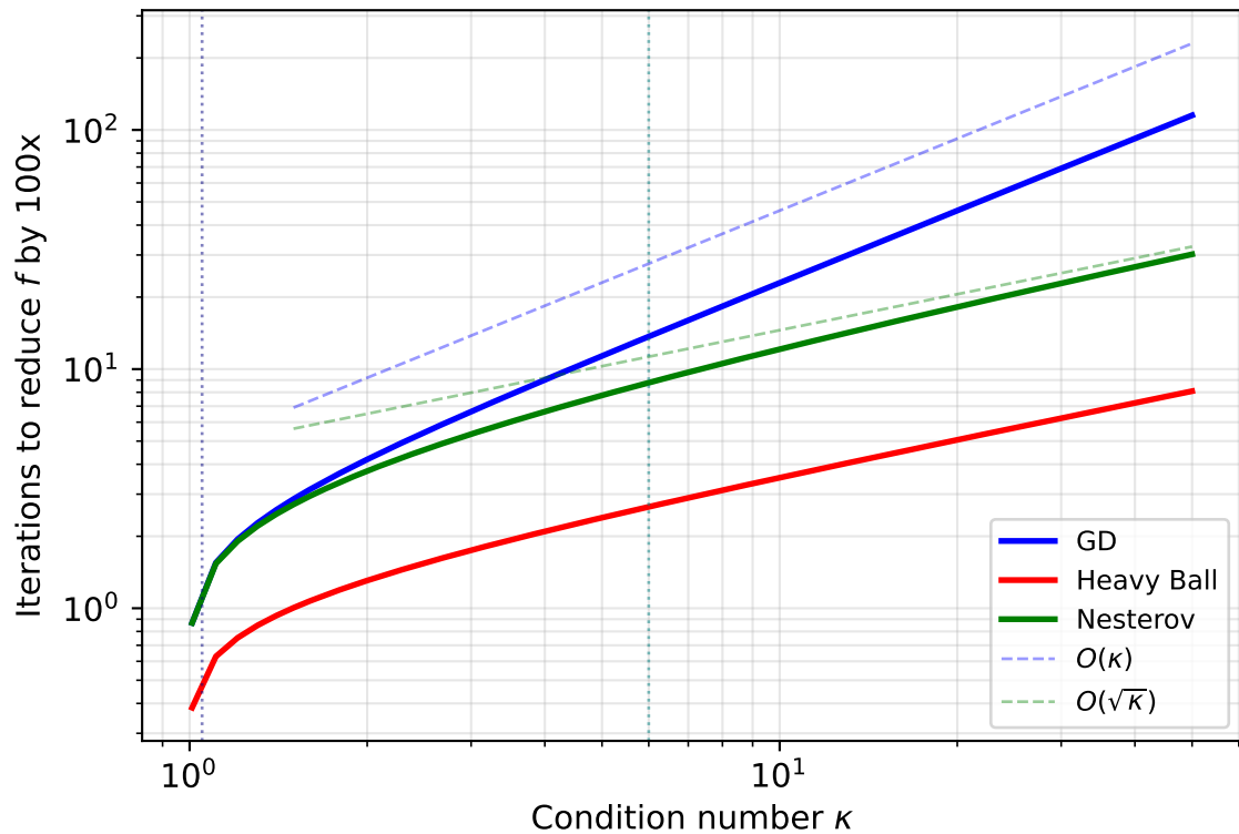
Iterations to Converge: O(\kappa) vs O(\sqrt{\kappa})
